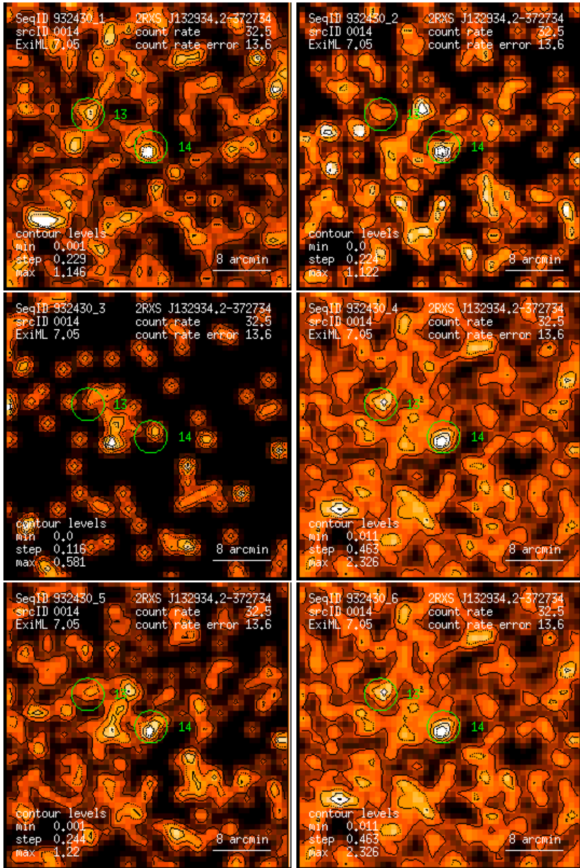
Figure 14: RASS 932430: detection 0014: band rate images, Gaussian filter: (1) PSPC channels 11 – 41, (2) 52 – 90, (3) 91 – 201, (4) 11 – 235, (5) 52 – 201, (6) 11 – 201. Broad band rates in counts/ks. Band rate contour levels in counts/ks/arcmin 2 .
