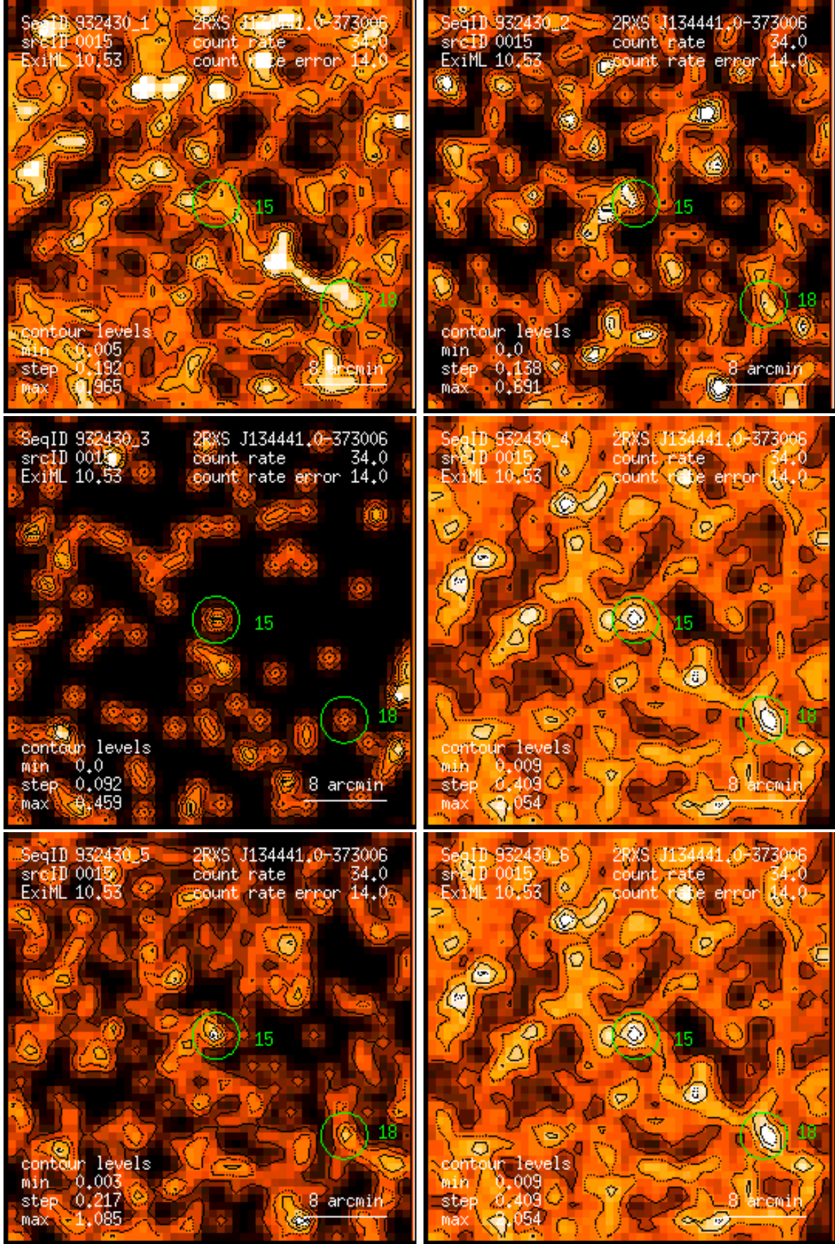
Figure 15: RASS 932430: detection 0015: band rate images, Gaussian filter: (1) PSPC channels 11 – 41, (2) 52 – 90, (3) 91 – 201, (4) 11 – 235, (5) 52 – 201, (6) 11 – 201. Broad band rates in counts/ks. Band rate contour levels in counts/ks/arcmin 2 .
