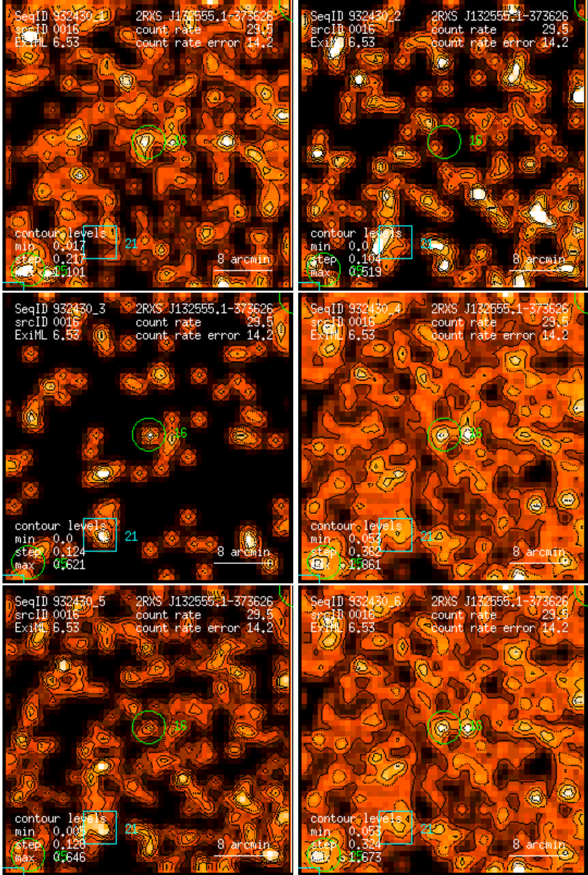
Figure 16: RASS 932430: detection 0016: band rate images, Gaussian filter: (1) PSPC channels 11 – 41, (2) 52 – 90, (3) 91 – 201, (4) 11 – 235, (5) 52 – 201, (6) 11 – 201. Broad band rates in counts/ks. Band rate contour levels in counts/ks/arcmin 2 .
