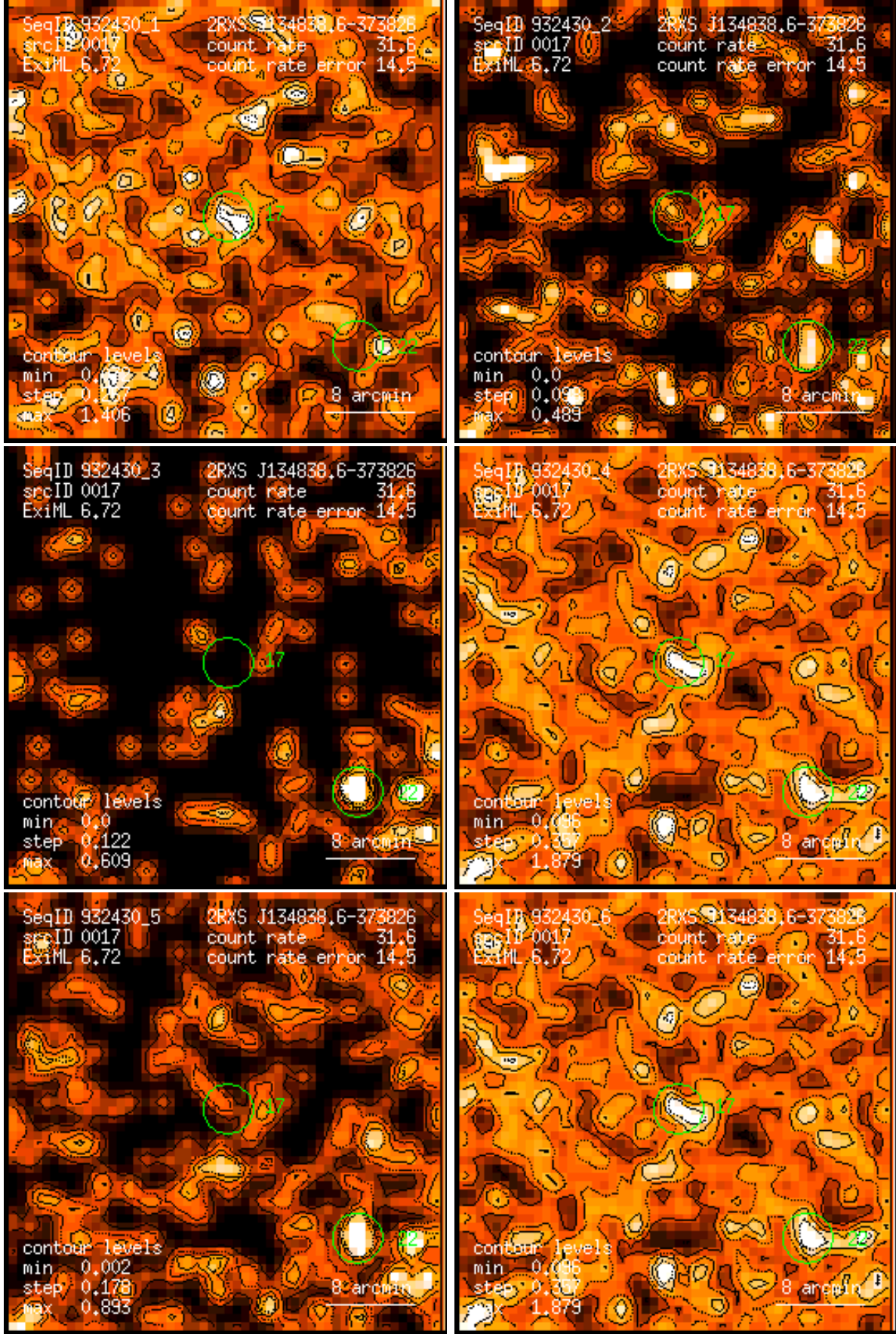
Figure 17: RASS 932430: detection 0017: band rate images, Gaussian filter: (1) PSPC channels 11 – 41, (2) 52 – 90, (3) 91 – 201, (4) 11 – 235, (5) 52 – 201, (6) 11 – 201. Broad band rates in counts/ks. Band rate contour levels in counts/ks/arcmin 2 .
