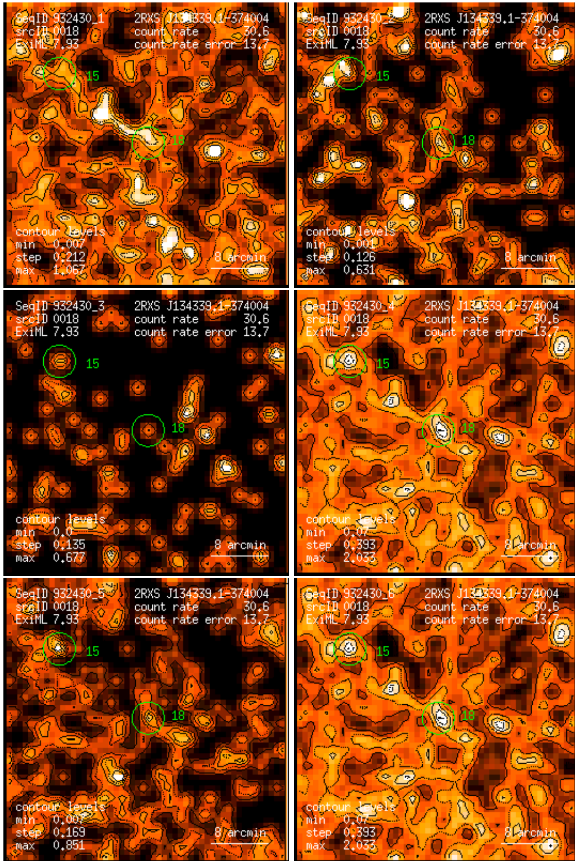
Figure 18: RASS 932430: detection 0018: band rate images, Gaussian filter: (1) PSPC channels 11 – 41, (2) 52 – 90, (3) 91 – 201, (4) 11 – 235, (5) 52 – 201, (6) 11 – 201. Broad band rates in counts/ks. Band rate contour levels in counts/ks/arcmin 2 .
