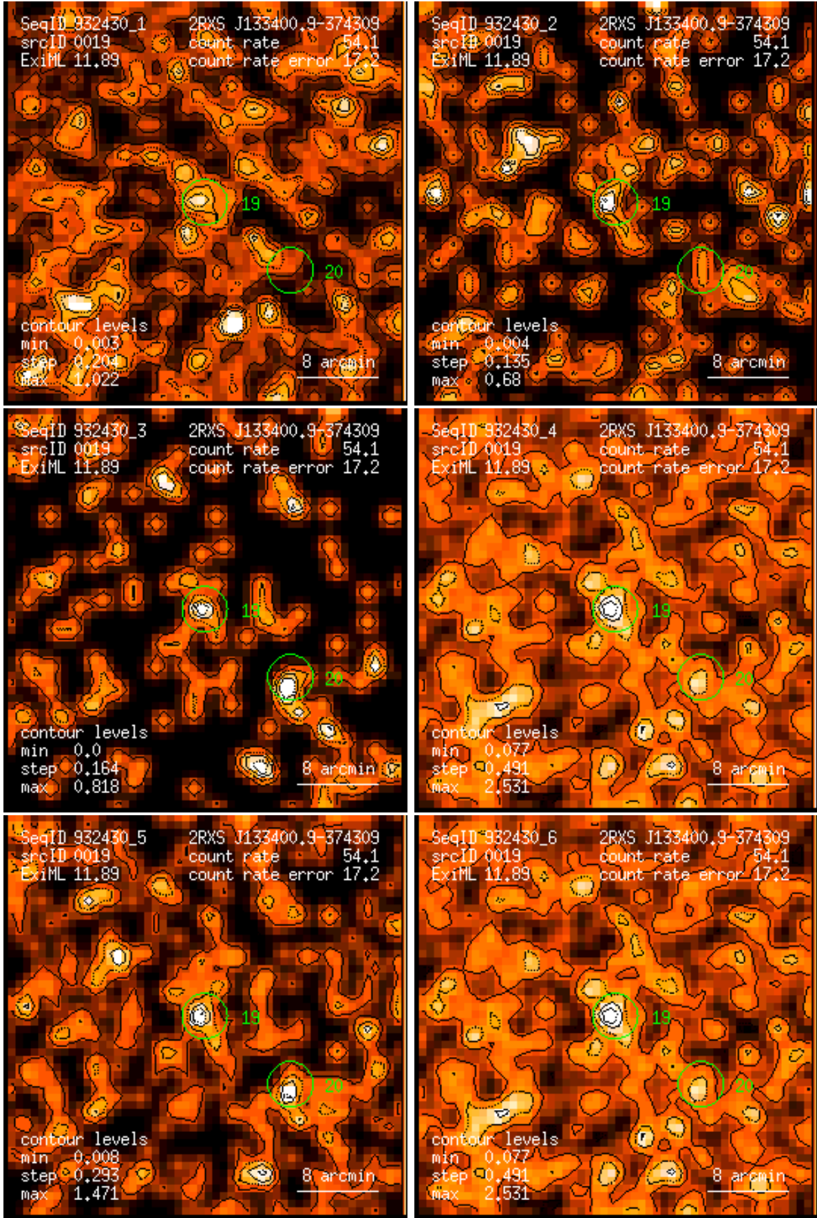
Figure 19: RASS 932430: detection 0019: band rate images, Gaussian filter: (1) PSPC channels 11 – 41, (2) 52 – 90, (3) 91 – 201, (4) 11 – 235, (5) 52 – 201, (6) 11 – 201. Broad band rates in counts/ks. Band rate contour levels in counts/ks/arcmin 2 .
