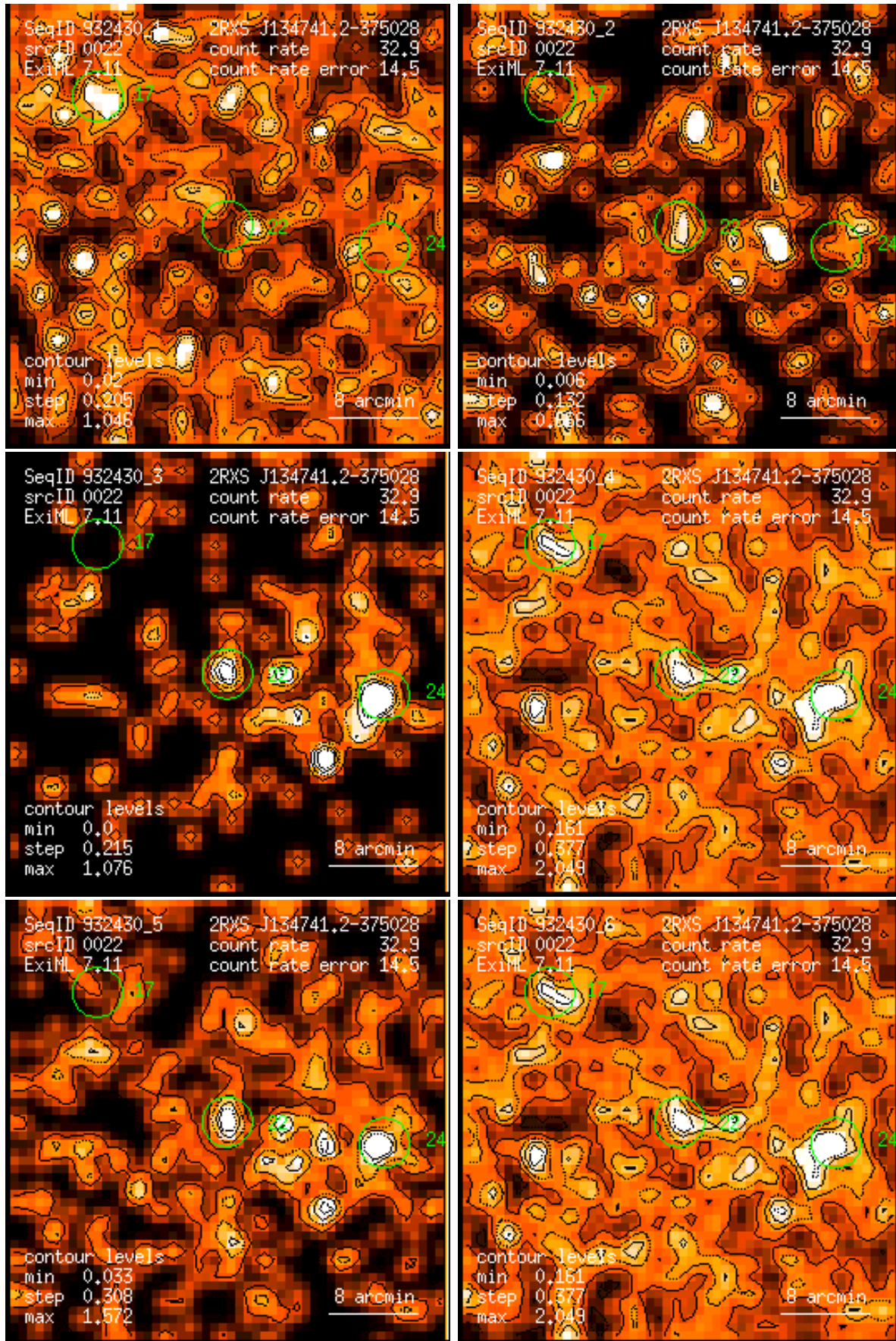
Figure 22: RASS 932430: detection 0022: band rate images, Gaussian filter: (1) PSPC channels 11 – 41, (2) 52 – 90, (3) 91 – 201, (4) 11 – 235, (5) 52 – 201, (6) 11 – 201. Broad band rates in counts/ks. Band rate contour levels in counts/ks/arcmin 2 .
