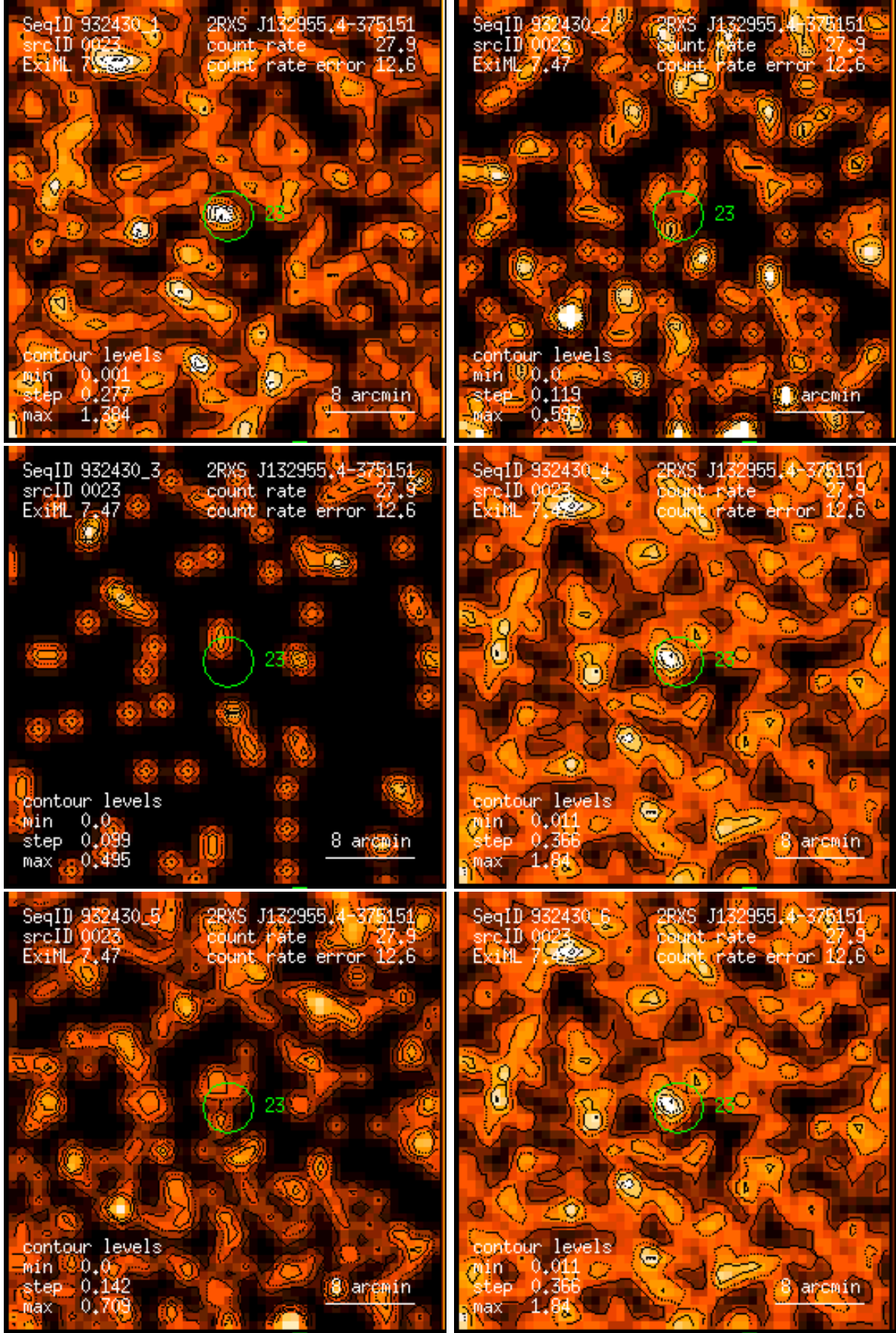
Figure 23: RASS 932430: detection 0023: band rate images, Gaussian filter: (1) PSPC channels 11 – 41, (2) 52 – 90, (3) 91 – 201, (4) 11 – 235, (5) 52 – 201, (6) 11 – 201. Broad band rates in counts/ks. Band rate contour levels in counts/ks/arcmin 2 .
