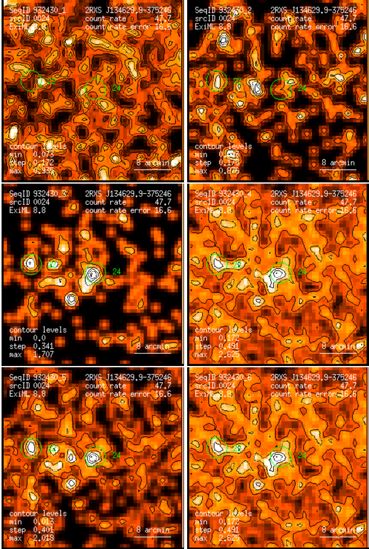
Figure 24: RASS 932430: detection 0024: band rate images, Gaussian filter: (1) PSPC channels 11 – 41, (2) 52 – 90, (3) 91 – 201, (4) 11 – 235, (5) 52 – 201, (6) 11 – 201. Broad band rates in counts/ks. Band rate contour levels in counts/ks/arcmin 2 .
