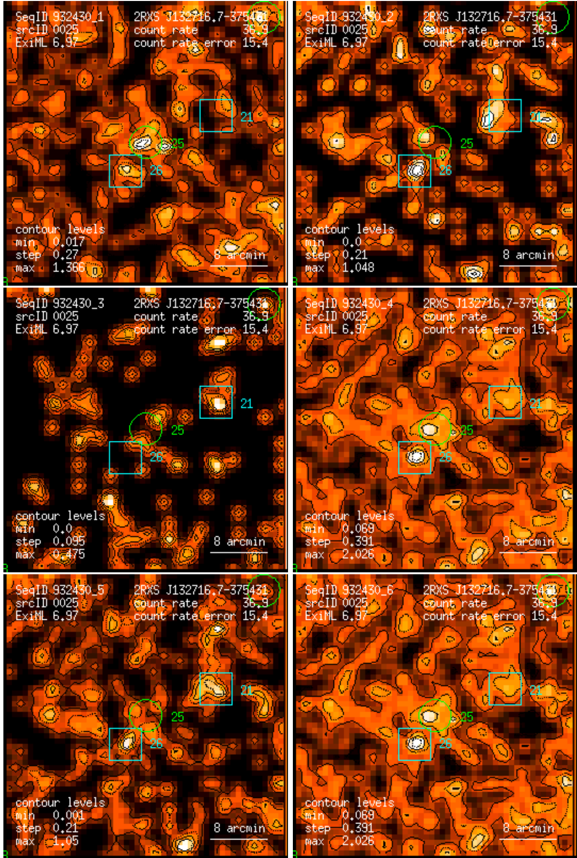
Figure 25: RASS 932430: detection 0025: band rate images, Gaussian filter: (1) PSPC channels 11 – 41, (2) 52 – 90, (3) 91 – 201, (4) 11 – 235, (5) 52 – 201, (6) 11 – 201. Broad band rates in counts/ks. Band rate contour levels in counts/ks/arcmin 2 .
