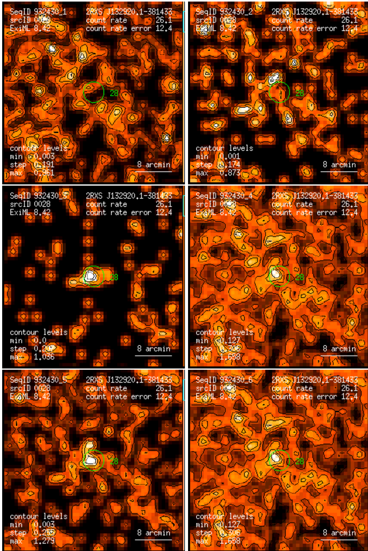
Figure 28: RASS 932430: detection 0028: band rate images, Gaussian filter: (1) PSPC channels 11 – 41, (2) 52 – 90, (3) 91 – 201, (4) 11 – 235, (5) 52 – 201, (6) 11 – 201. Broad band rates in counts/ks. Band rate contour levels in counts/ks/arcmin 2 .
