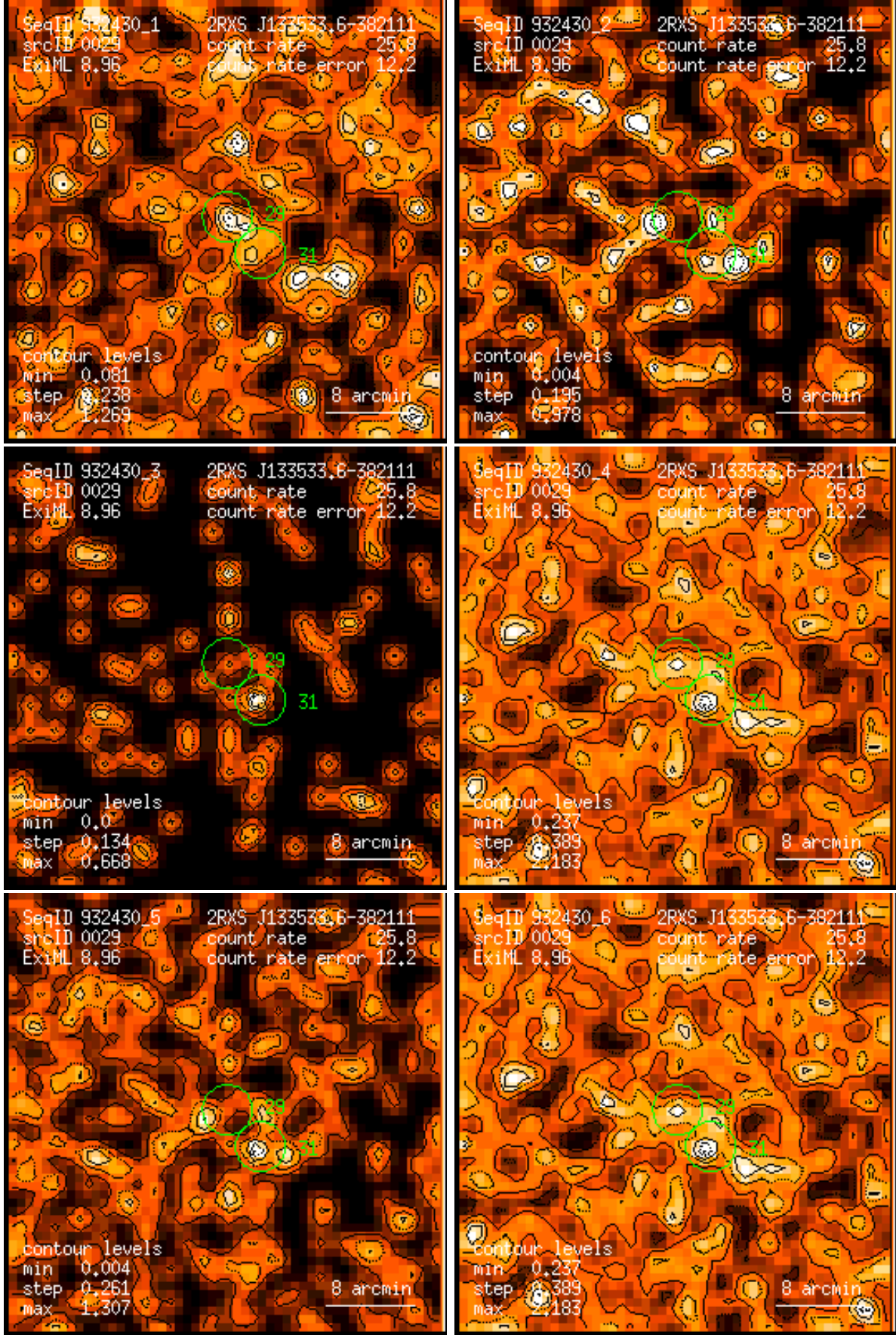
Figure 29: RASS 932430: detection 0029: band rate images, Gaussian filter: (1) PSPC channels 11 – 41, (2) 52 – 90, (3) 91 – 201, (4) 11 – 235, (5) 52 – 201, (6) 11 – 201. Broad band rates in counts/ks. Band rate contour levels in counts/ks/arcmin 2 .
