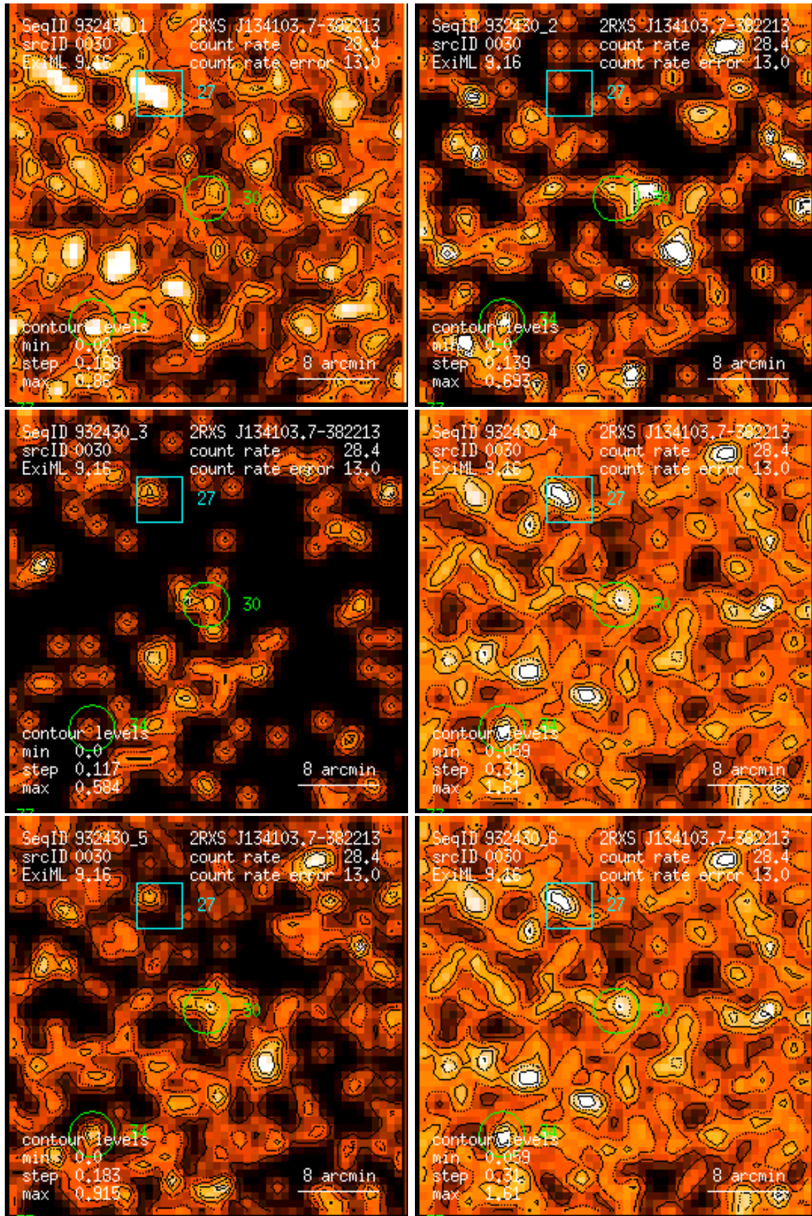
Figure 30: RASS 932430: detection 0030: band rate images, Gaussian filter: (1) PSPC channels 11 – 41, (2) 52 – 90, (3) 91 – 201, (4) 11 – 235, (5) 52 – 201, (6) 11 – 201. Broad band rates in counts/ks. Band rate contour levels in counts/ks/arcmin 2 .
