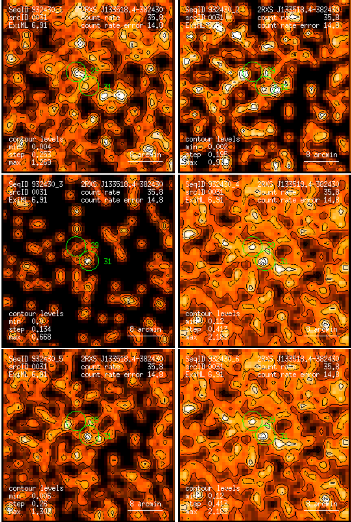
Figure 31: RASS 932430: detection 0031: band rate images, Gaussian filter: (1) PSPC channels 11 – 41, (2) 52 – 90, (3) 91 – 201, (4) 11 – 235, (5) 52 – 201, (6) 11 – 201. Broad band rates in counts/ks. Band rate contour levels in counts/ks/arcmin 2 .
