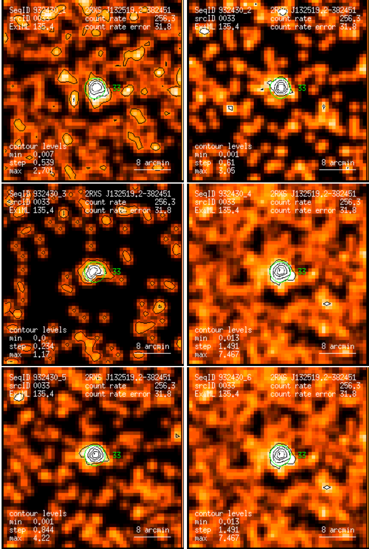
Figure 33: RASS 932430: detection 0033: band rate images, Gaussian filter: (1) PSPC channels 11 – 41, (2) 52 – 90, (3) 91 – 201, (4) 11 – 235, (5) 52 – 201, (6) 11 – 201. Broad band rates in counts/ks. Band rate contour levels in counts/ks/arcmin 2 .
