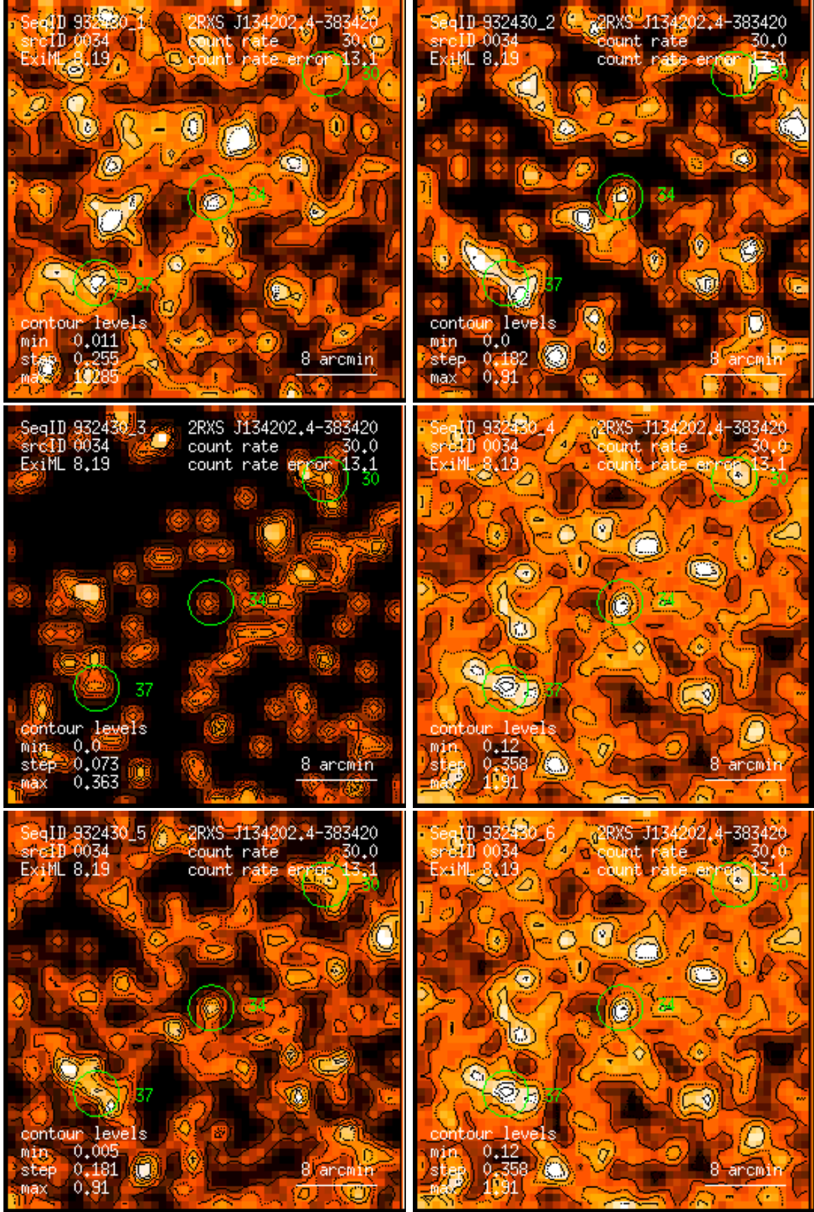
Figure 34: RASS 932430: detection 0034: band rate images, Gaussian filter: (1) PSPC channels 11 – 41, (2) 52 – 90, (3) 91 – 201, (4) 11 – 235, (5) 52 – 201, (6) 11 – 201. Broad band rates in counts/ks. Band rate contour levels in counts/ks/arcmin 2 .
