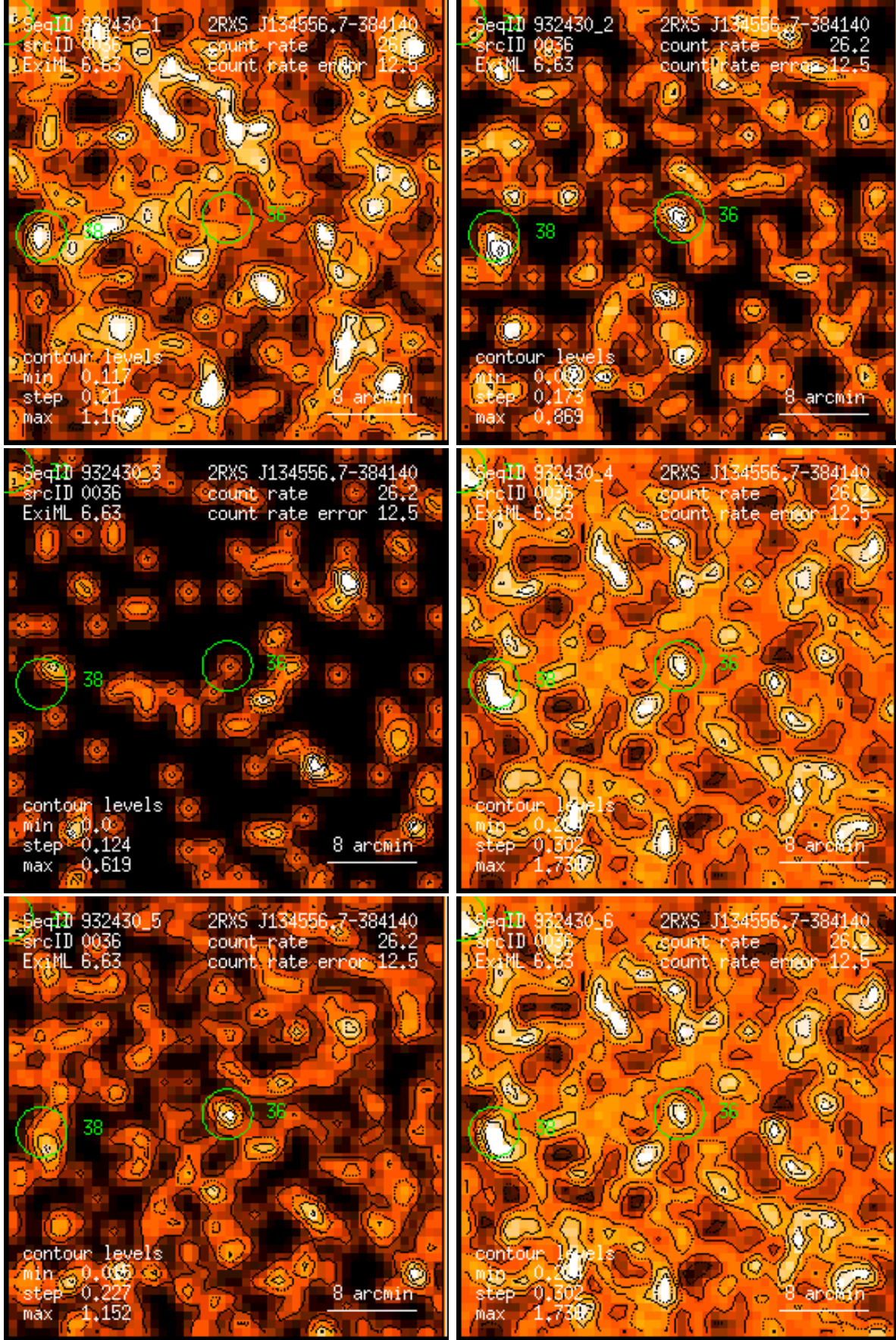
Figure 36: RASS 932430: detection 0036: band rate images, Gaussian filter: (1) PSPC channels 11 – 41, (2) 52 – 90, (3) 91 – 201, (4) 11 – 235, (5) 52 – 201, (6) 11 – 201. Broad band rates in counts/ks. Band rate contour levels in counts/ks/arcmin 2 .
