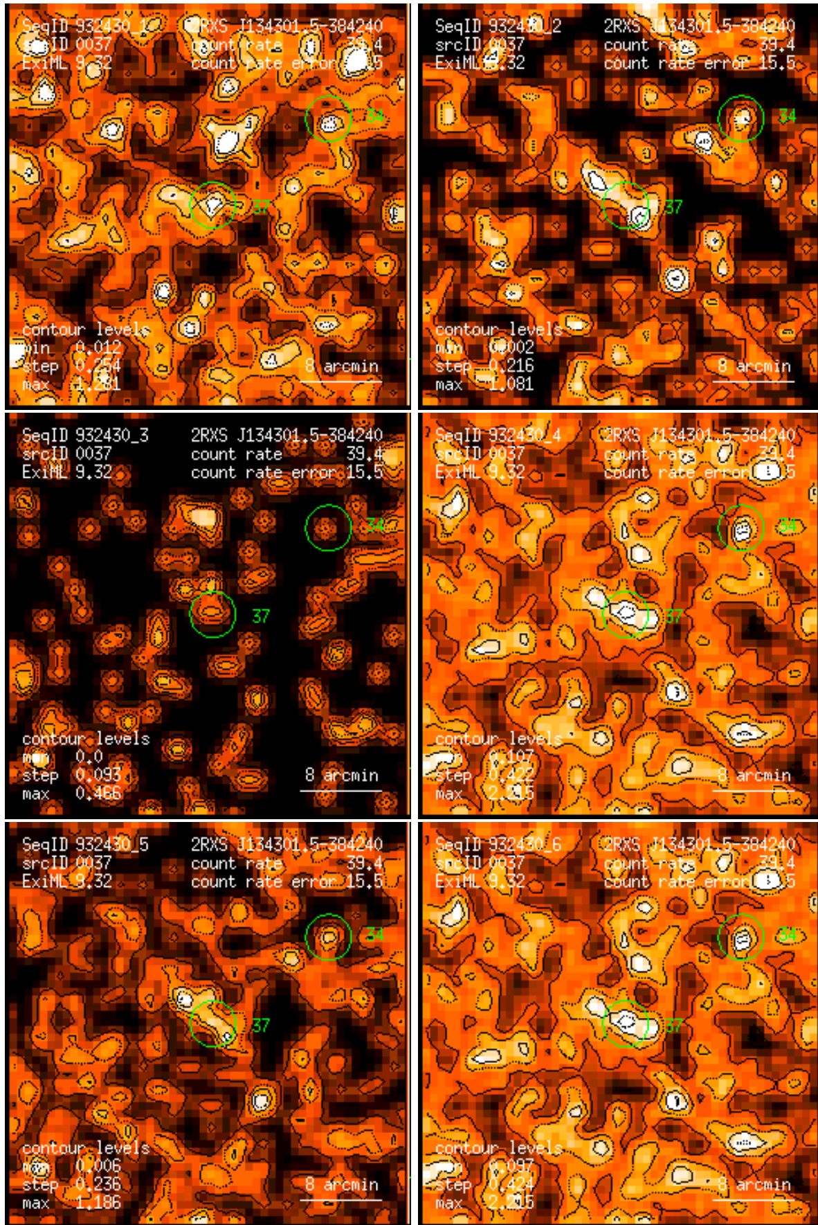
Figure 37: RASS 932430: detection 0037: band rate images, Gaussian filter: (1) PSPC channels 11 – 41, (2) 52 – 90, (3) 91 – 201, (4) 11 – 235, (5) 52 – 201, (6) 11 – 201. Broad band rates in counts/ks. Band rate contour levels in counts/ks/arcmin 2 .
