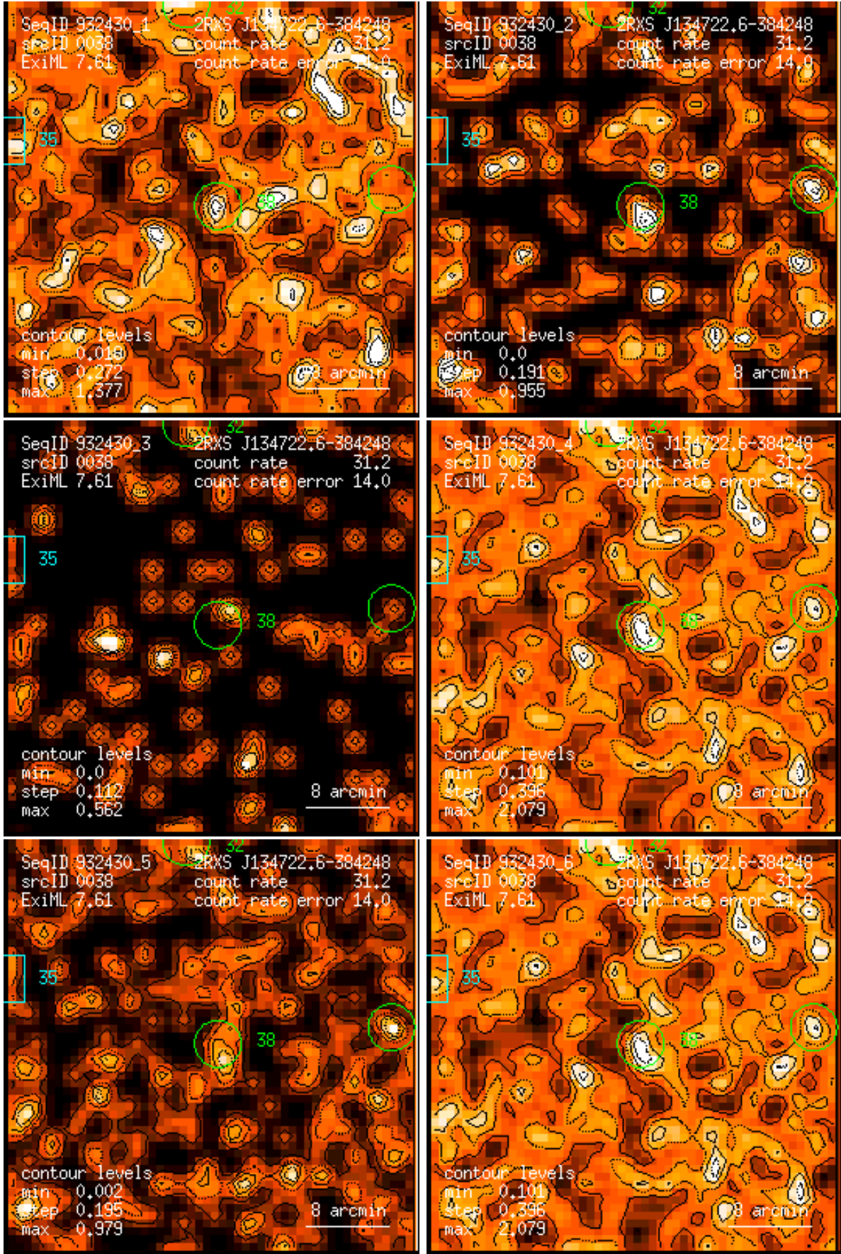
Figure 38: RASS 932430: detection 0038: band rate images, Gaussian filter: (1) PSPC channels 11 – 41, (2) 52 – 90, (3) 91 – 201, (4) 11 – 235, (5) 52 – 201, (6) 11 – 201. Broad band rates in counts/ks. Band rate contour levels in counts/ks/arcmin 2 .
