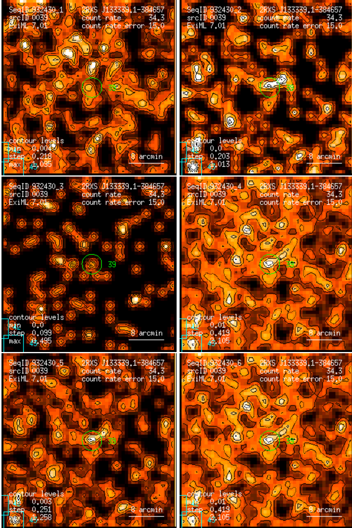
Figure 39: RASS 932430: detection 0039: band rate images, Gaussian filter: (1) PSPC channels 11 – 41, (2) 52 – 90, (3) 91 – 201, (4) 11 – 235, (5) 52 – 201, (6) 11 – 201. Broad band rates in counts/ks. Band rate contour levels in counts/ks/arcmin 2 .
