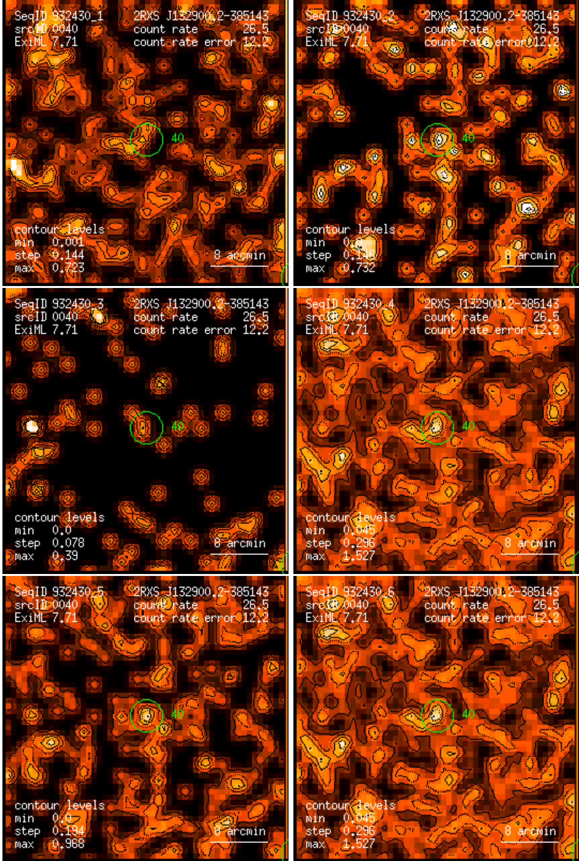
Figure 40: RASS 932430: detection 0040: band rate images, Gaussian filter: (1) PSPC channels 11 – 41, (2) 52 – 90, (3) 91 – 201, (4) 11 – 235, (5) 52 – 201, (6) 11 – 201. Broad band rates in counts/ks. Band rate contour levels in counts/ks/arcmin 2 .
