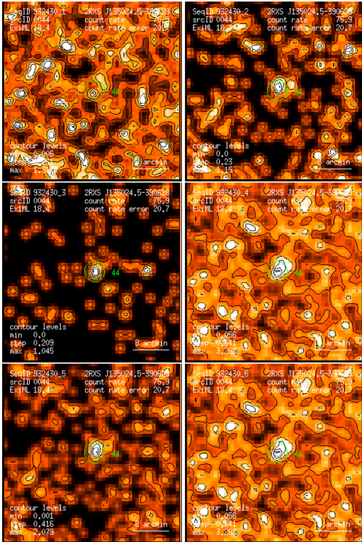
Figure 44: RASS 932430: detection 0044: band rate images, Gaussian filter: (1) PSPC channels 11 – 41, (2) 52 – 90, (3) 91 – 201, (4) 11 – 235, (5) 52 – 201, (6) 11 – 201. Broad band rates in counts/ks. Band rate contour levels in counts/ks/arcmin 2 .
