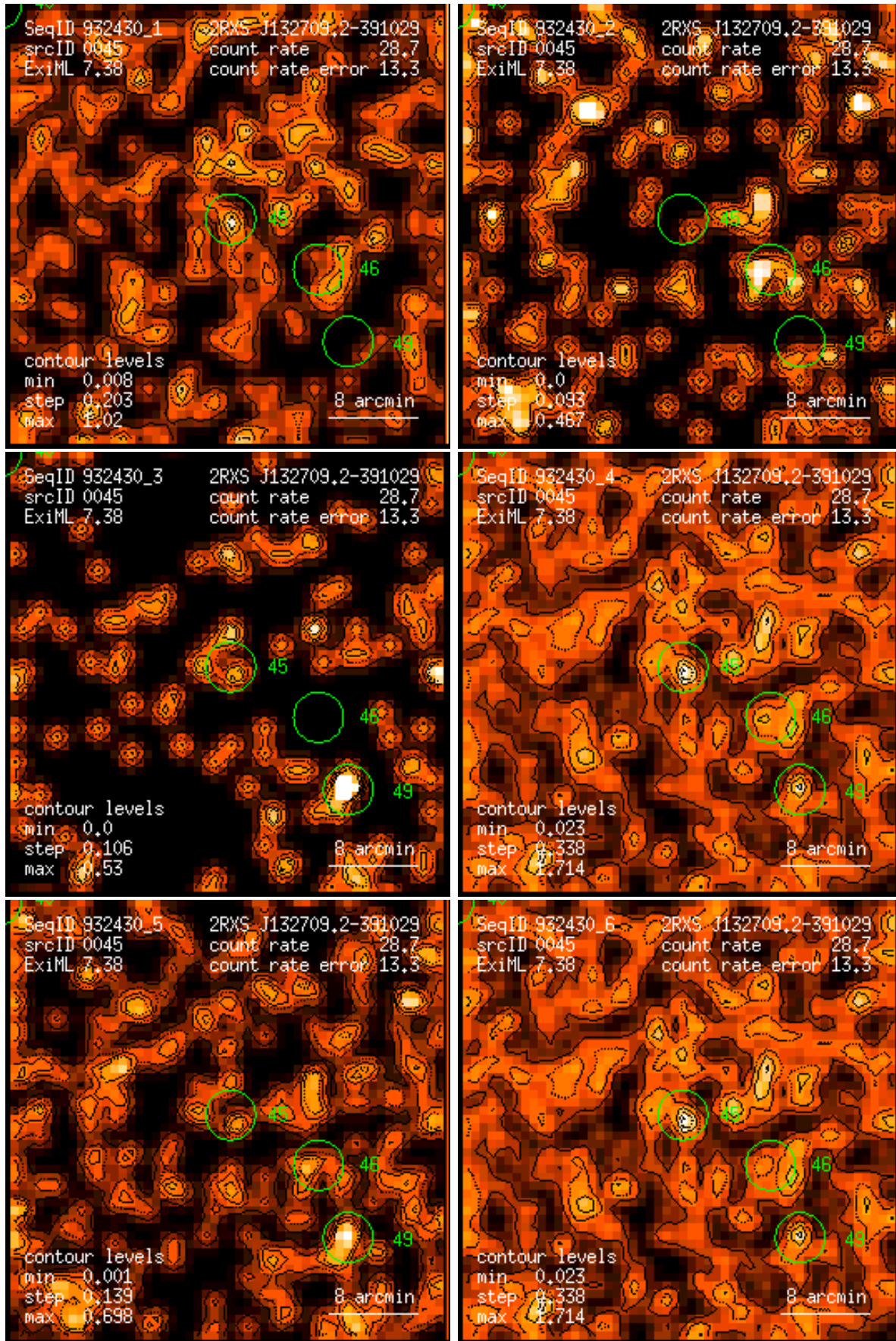
Figure 45: RASS 932430: detection 0045: band rate images, Gaussian filter: (1) PSPC channels 11 – 41, (2) 52 – 90, (3) 91 – 201, (4) 11 – 235, (5) 52 – 201, (6) 11 – 201. Broad band rates in counts/ks. Band rate contour levels in counts/ks/arcmin 2 .
