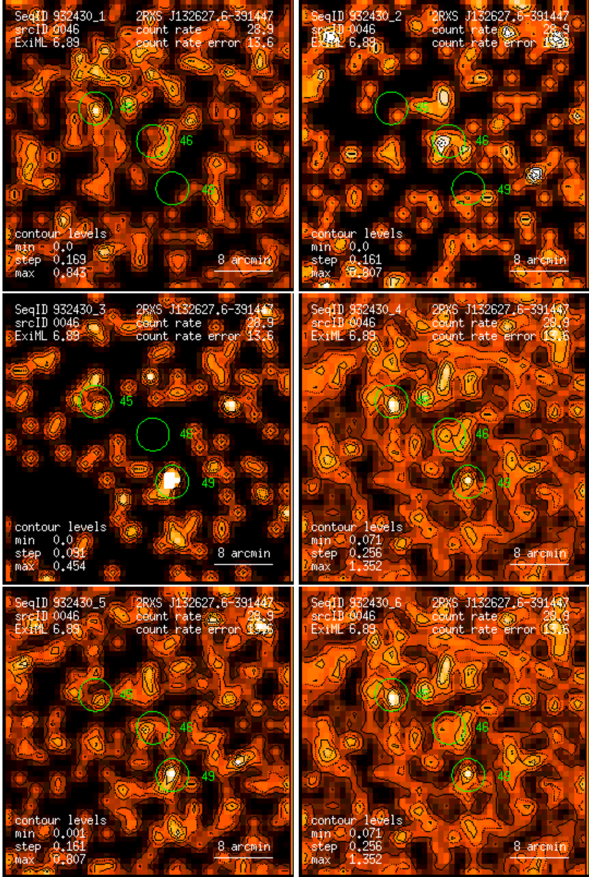
Figure 46: RASS 932430: detection 0046: band rate images, Gaussian filter: (1) PSPC channels 11 – 41, (2) 52 – 90, (3) 91 – 201, (4) 11 – 235, (5) 52 – 201, (6) 11 – 201. Broad band rates in counts/ks. Band rate contour levels in counts/ks/arcmin 2 .
