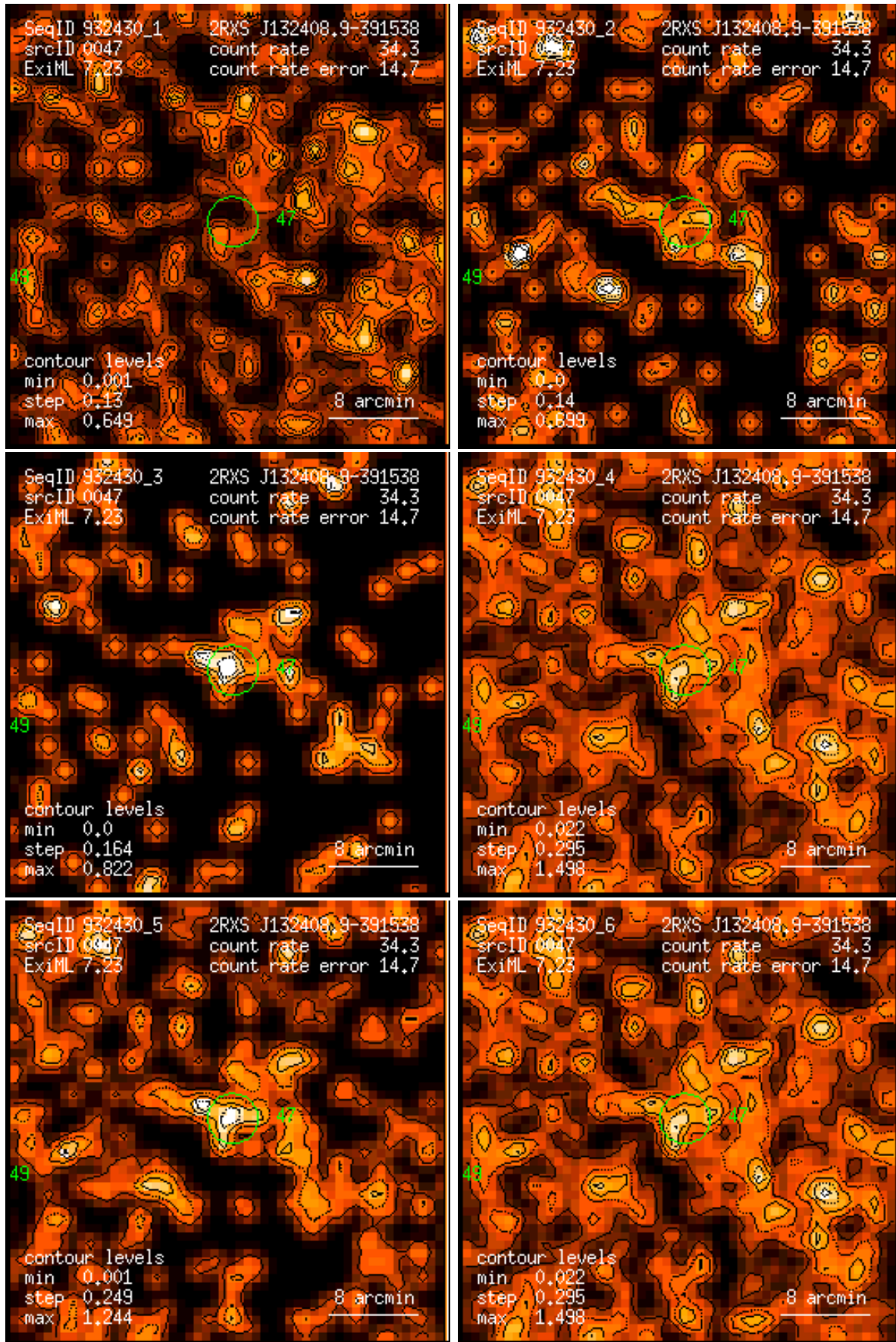
Figure 47: RASS 932430: detection 0047: band rate images, Gaussian filter: (1) PSPC channels 11 – 41, (2) 52 – 90, (3) 91 – 201, (4) 11 – 235, (5) 52 – 201, (6) 11 – 201. Broad band rates in counts/ks. Band rate contour levels in counts/ks/arcmin 2 .
