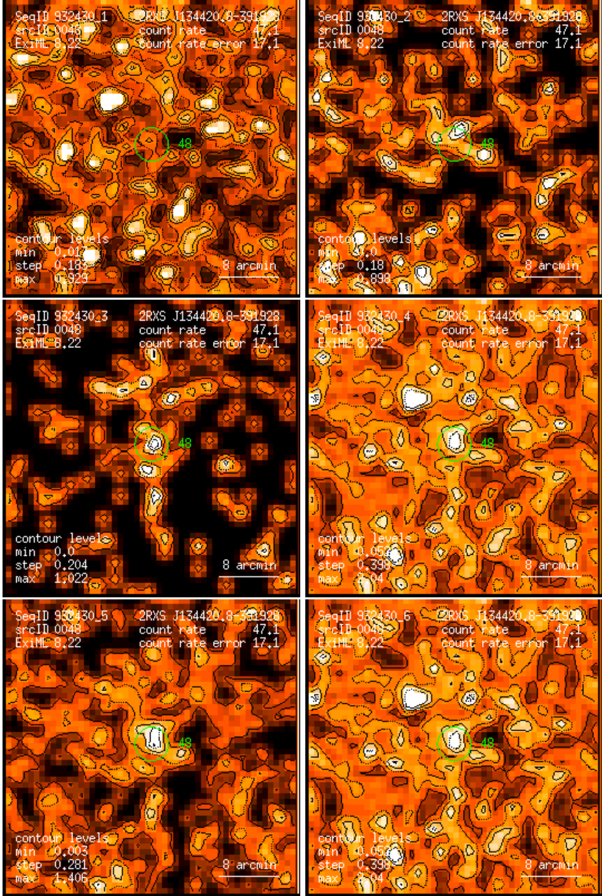
Figure 48: RASS 932430: detection 0048: band rate images, Gaussian filter: (1) PSPC channels 11 – 41, (2) 52 – 90, (3) 91 – 201, (4) 11 – 235, (5) 52 – 201, (6) 11 – 201. Broad band rates in counts/ks. Band rate contour levels in counts/ks/arcmin 2 .
