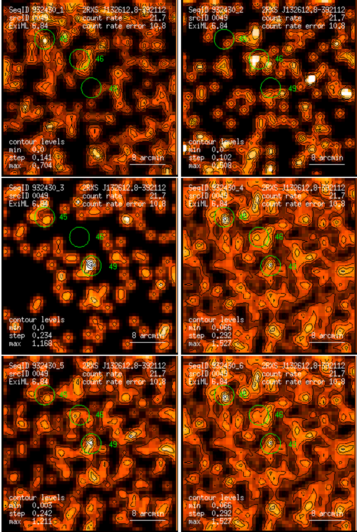
Figure 49: RASS 932430: detection 0049: band rate images, Gaussian filter: (1) PSPC channels 11 – 41, (2) 52 – 90, (3) 91 – 201, (4) 11 – 235, (5) 52 – 201, (6) 11 – 201. Broad band rates in counts/ks. Band rate contour levels in counts/ks/arcmin 2 .
