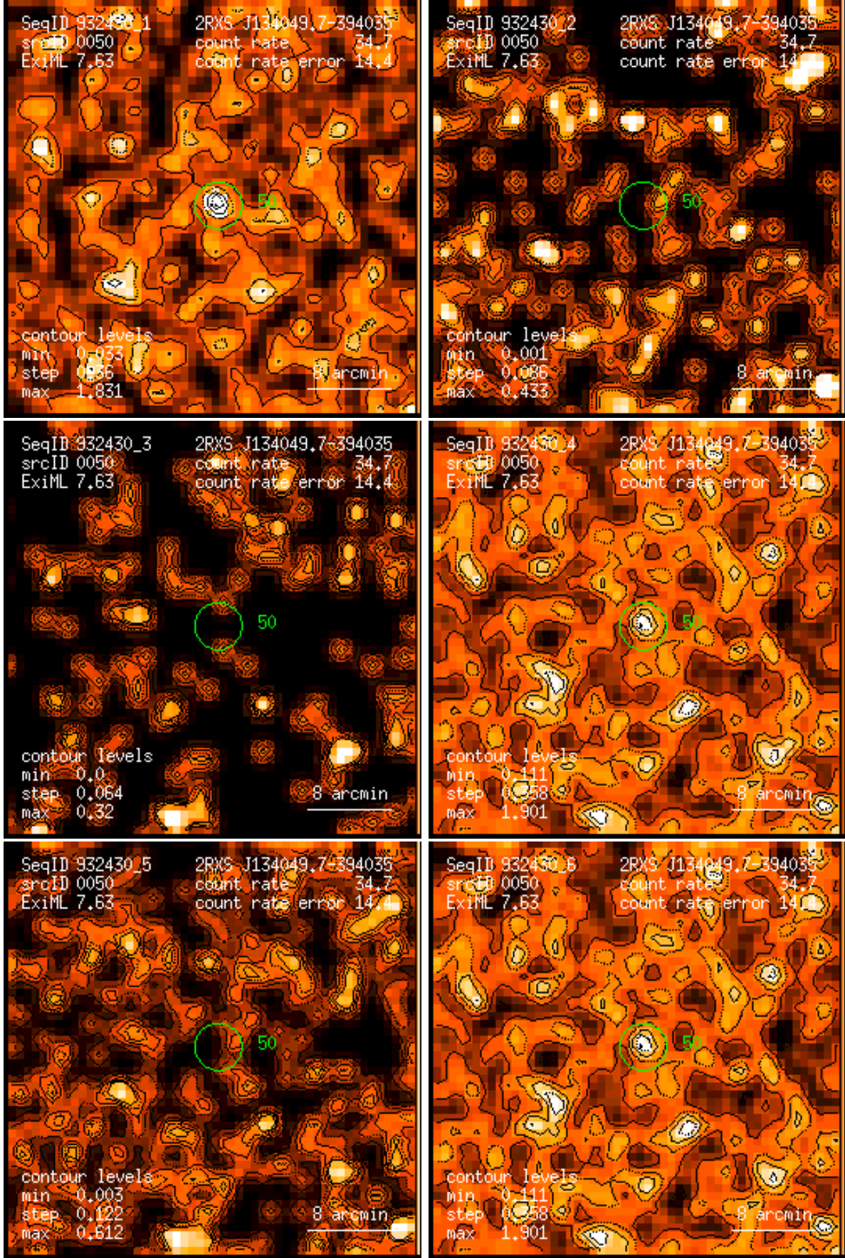
Figure 50: RASS 932430: detection 0050: band rate images, Gaussian filter: (1) PSPC channels 11 – 41, (2) 52 – 90, (3) 91 – 201, (4) 11 – 235, (5) 52 – 201, (6) 11 – 201. Broad band rates in counts/ks. Band rate contour levels in counts/ks/arcmin 2 .
