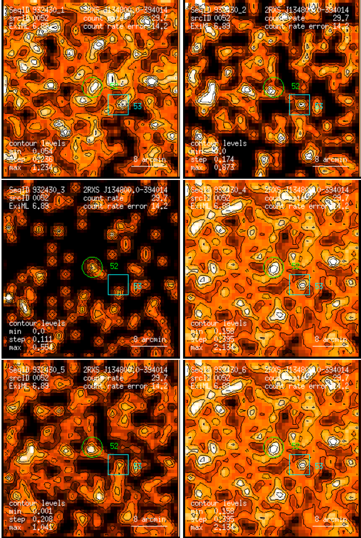
Figure 52: RASS 932430: detection 0052: band rate images, Gaussian filter: (1) PSPC channels 11 – 41, (2) 52 – 90, (3) 91 – 201, (4) 11 – 235, (5) 52 – 201, (6) 11 – 201. Broad band rates in counts/ks. Band rate contour levels in counts/ks/arcmin 2 .
