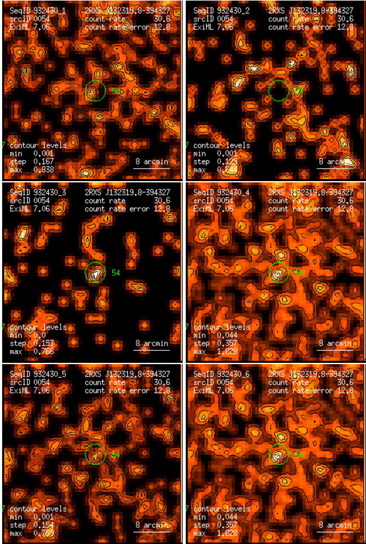
Figure 54: RASS 932430: detection 0054: band rate images, Gaussian filter: (1) PSPC channels 11 – 41, (2) 52 – 90, (3) 91 – 201, (4) 11 – 235, (5) 52 – 201, (6) 11 – 201. Broad band rates in counts/ks. Band rate contour levels in counts/ks/arcmin 2 .
