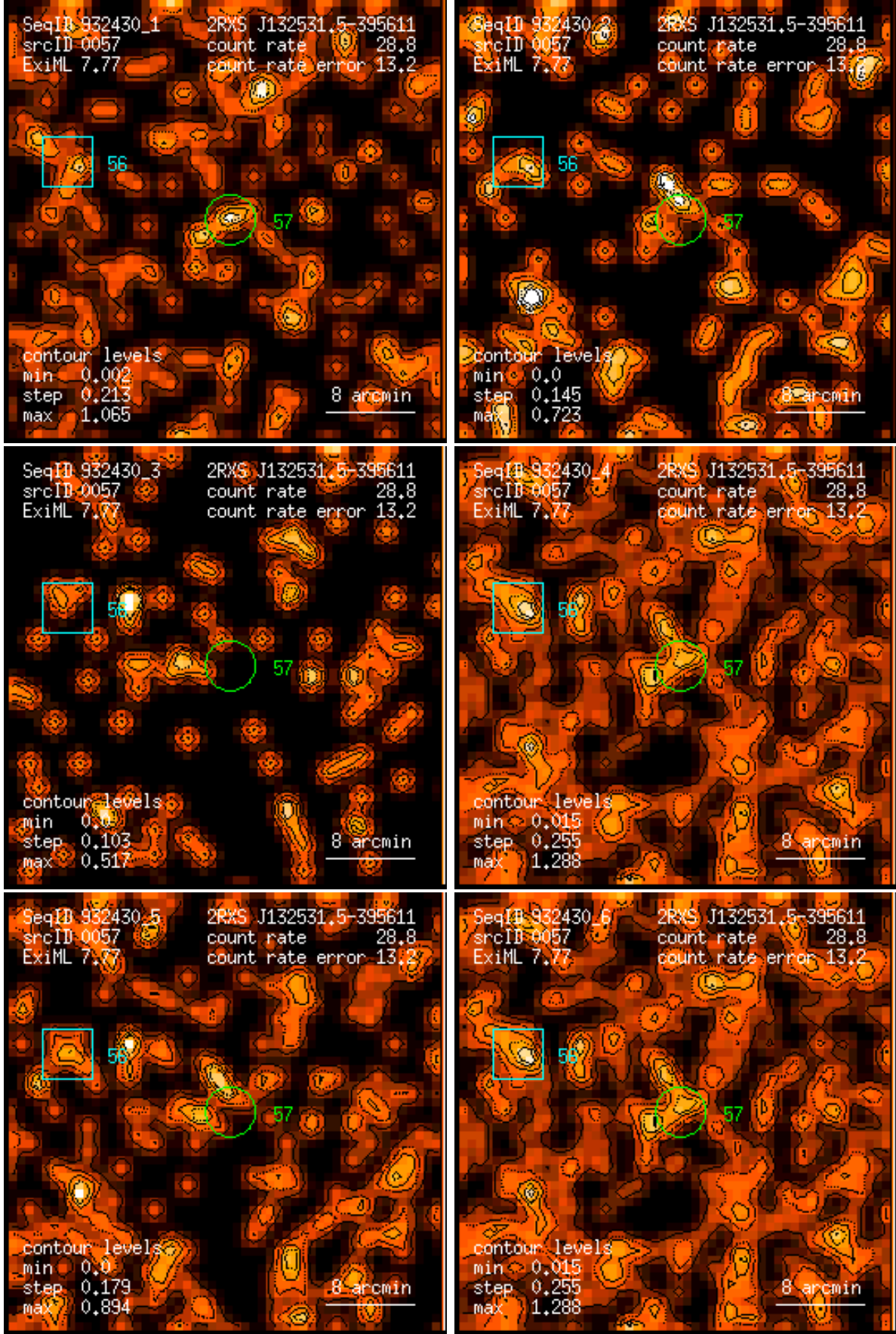
Figure 57: RASS 932430: detection 0057: band rate images, Gaussian filter: (1) PSPC channels 11 – 41, (2) 52 – 90, (3) 91 – 201, (4) 11 – 235, (5) 52 – 201, (6) 11 – 201. Broad band rates in counts/ks. Band rate contour levels in counts/ks/arcmin 2 .
