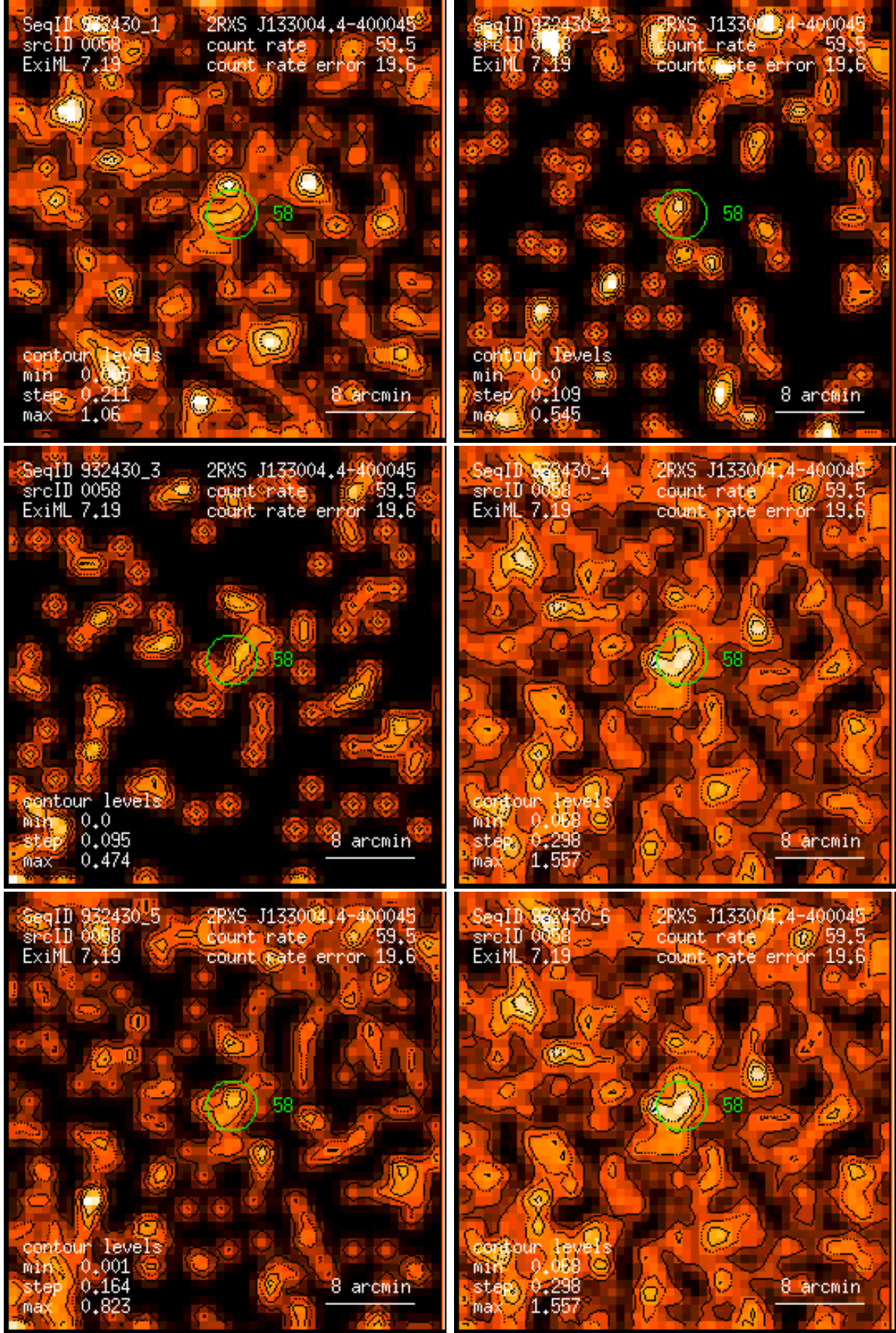
Figure 58: RASS 932430: detection 0058: band rate images, Gaussian filter: (1) PSPC channels 11 – 41, (2) 52 – 90, (3) 91 – 201, (4) 11 – 235, (5) 52 – 201, (6) 11 – 201. Broad band rates in counts/ks. Band rate contour levels in counts/ks/arcmin 2 .
