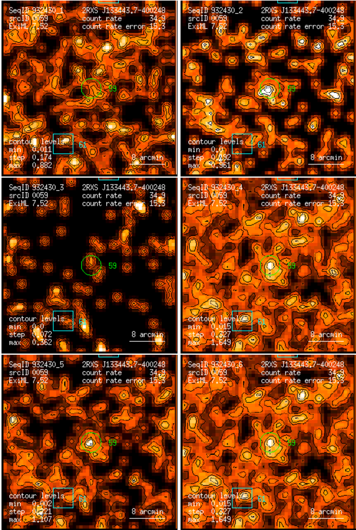
Figure 59: RASS 932430: detection 0059: band rate images, Gaussian filter: (1) PSPC channels 11 – 41, (2) 52 – 90, (3) 91 – 201, (4) 11 – 235, (5) 52 – 201, (6) 11 – 201. Broad band rates in counts/ks. Band rate contour levels in counts/ks/arcmin 2 .
