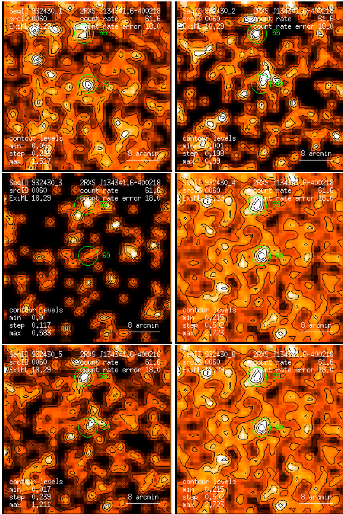
Figure 60: RASS 932430: detection 0060: band rate images, Gaussian filter: (1) PSPC channels 11 – 41, (2) 52 – 90, (3) 91 – 201, (4) 11 – 235, (5) 52 – 201, (6) 11 – 201. Broad band rates in counts/ks. Band rate contour levels in counts/ks/arcmin 2 .
