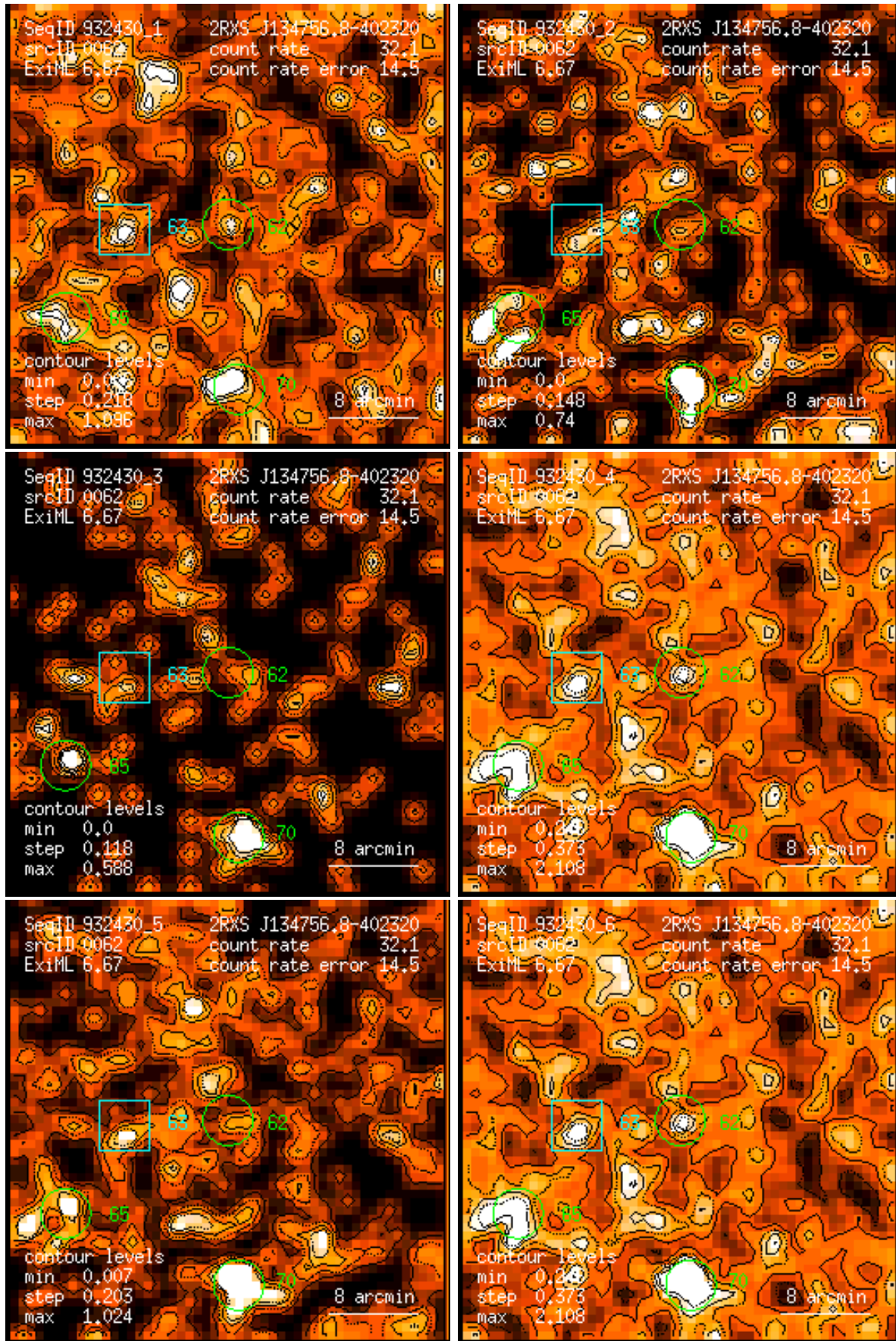
Figure 62: RASS 932430: detection 0062: band rate images, Gaussian filter: (1) PSPC channels 11 – 41, (2) 52 – 90, (3) 91 – 201, (4) 11 – 235, (5) 52 – 201, (6) 11 – 201. Broad band rates in counts/ks. Band rate contour levels in counts/ks/arcmin 2 .
