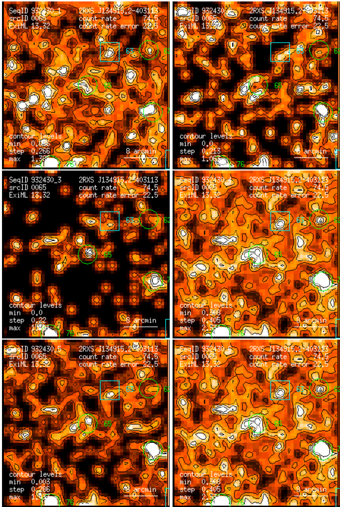
Figure 65: RASS 932430: detection 0065: band rate images, Gaussian filter: (1) PSPC channels 11 – 41, (2) 52 – 90, (3) 91 – 201, (4) 11 – 235, (5) 52 – 201, (6) 11 – 201. Broad band rates in counts/ks. Band rate contour levels in counts/ks/arcmin 2 .
