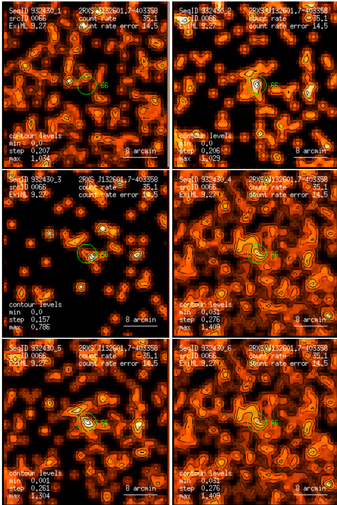
Figure 66: RASS 932430: detection 0066: band rate images, Gaussian filter: (1) PSPC channels 11 – 41, (2) 52 – 90, (3) 91 – 201, (4) 11 – 235, (5) 52 – 201, (6) 11 – 201. Broad band rates in counts/ks. Band rate contour levels in counts/ks/arcmin 2 .
