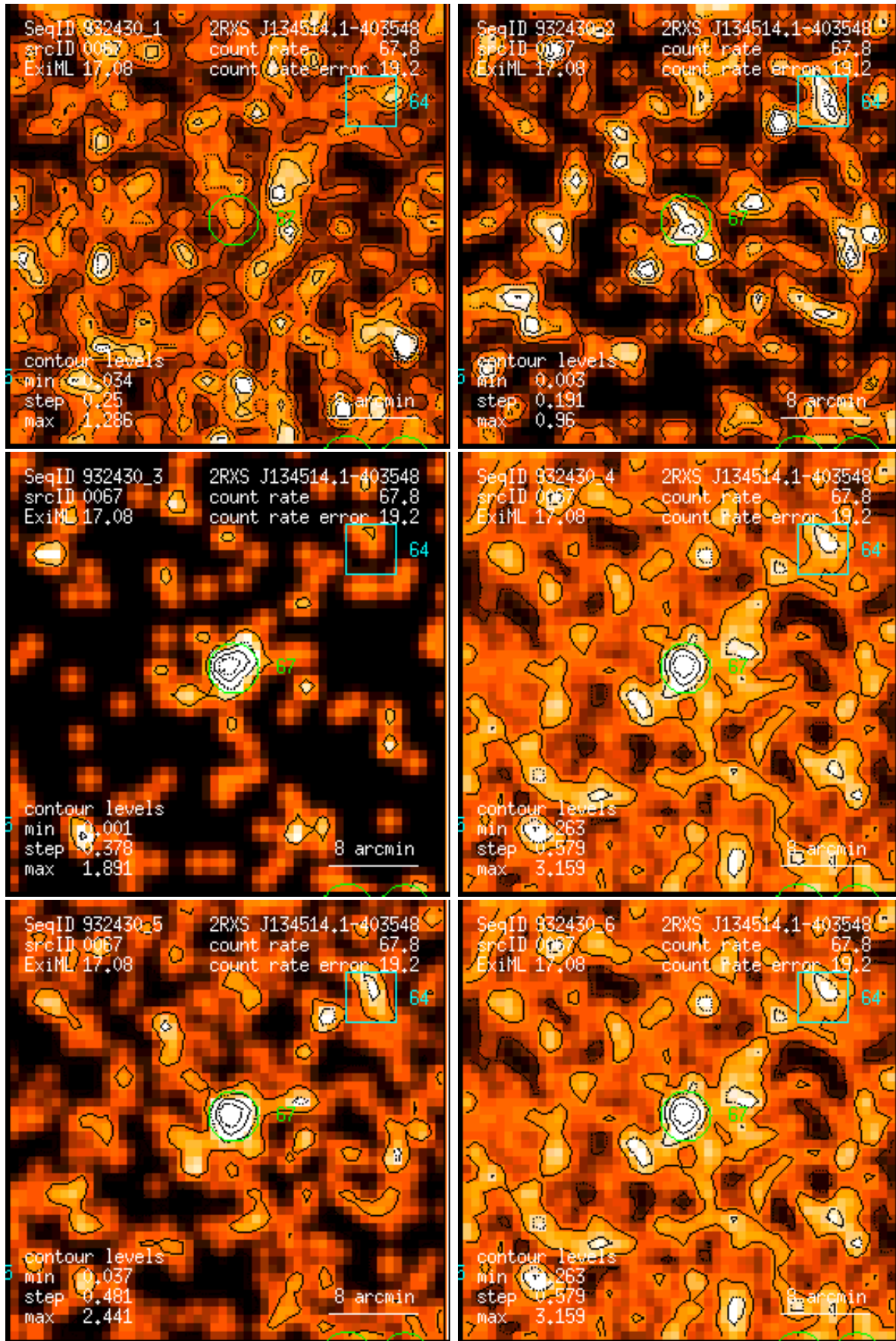
Figure 67: RASS 932430: detection 0067: band rate images, Gaussian filter: (1) PSPC channels 11 – 41, (2) 52 – 90, (3) 91 – 201, (4) 11 – 235, (5) 52 – 201, (6) 11 – 201. Broad band rates in counts/ks. Band rate contour levels in counts/ks/arcmin 2 .
