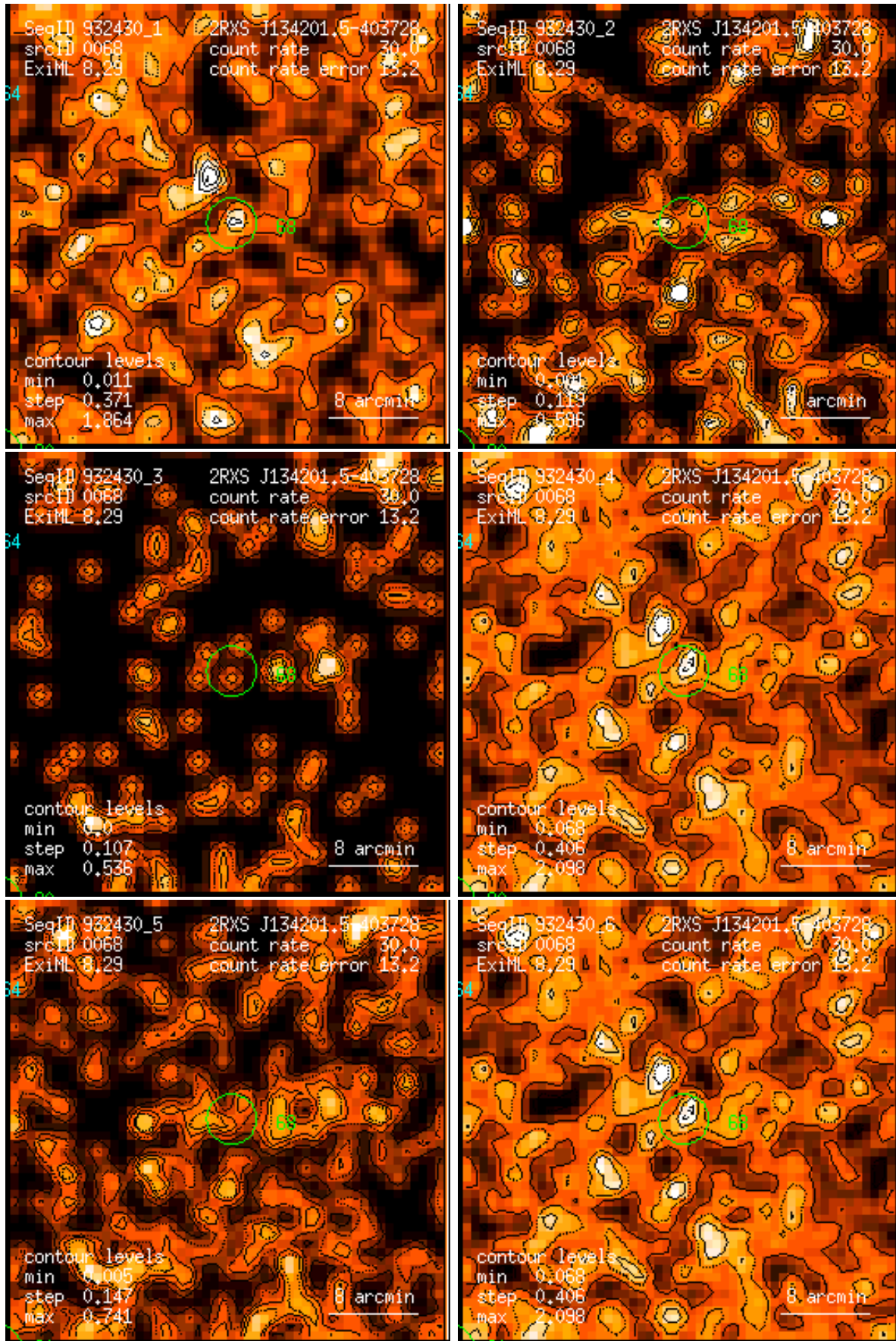
Figure 68: RASS 932430: detection 0068: band rate images, Gaussian filter: (1) PSPC channels 11 – 41, (2) 52 – 90, (3) 91 – 201, (4) 11 – 235, (5) 52 – 201, (6) 11 – 201. Broad band rates in counts/ks. Band rate contour levels in counts/ks/arcmin 2 .
