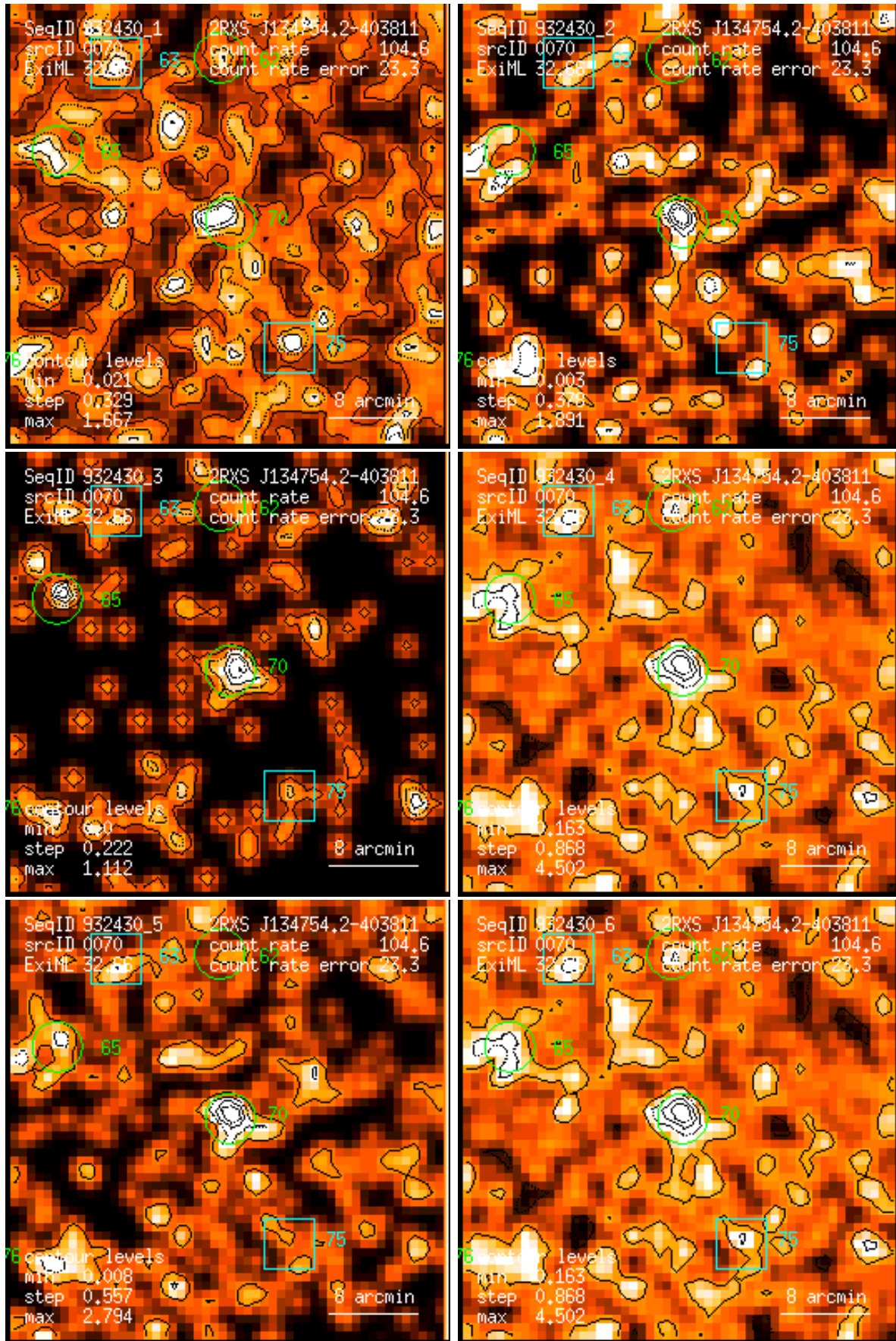
Figure 70: RASS 932430: detection 0070: band rate images, Gaussian filter: (1) PSPC channels 11 – 41, (2) 52 – 90, (3) 91 – 201, (4) 11 – 235, (5) 52 – 201, (6) 11 – 201. Broad band rates in counts/ks. Band rate contour levels in counts/ks/arcmin 2 .
