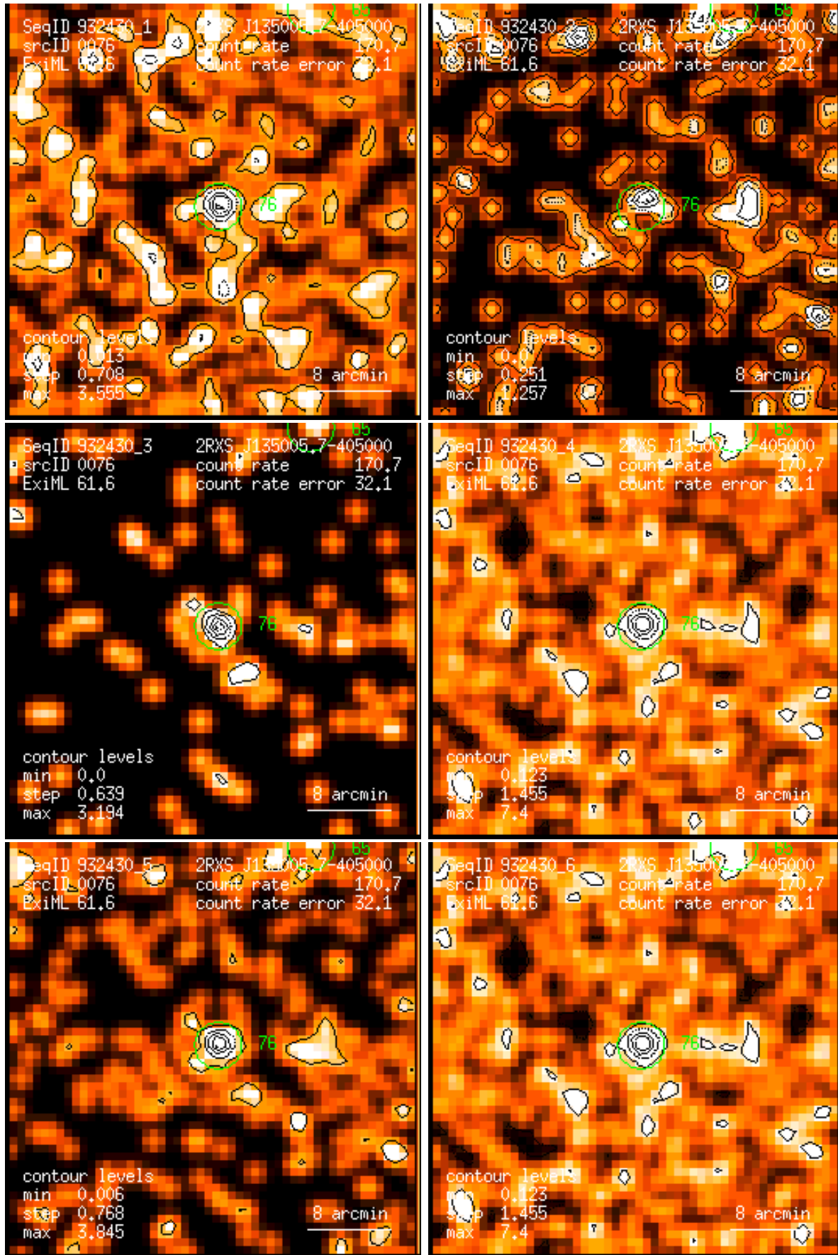
Figure 76: RASS 932430: detection 0076: band rate images, Gaussian filter: (1) PSPC channels 11 – 41, (2) 52 – 90, (3) 91 – 201, (4) 11 – 235, (5) 52 – 201, (6) 11 – 201. Broad band rates in counts/ks. Band rate contour levels in counts/ks/arcmin 2 .
