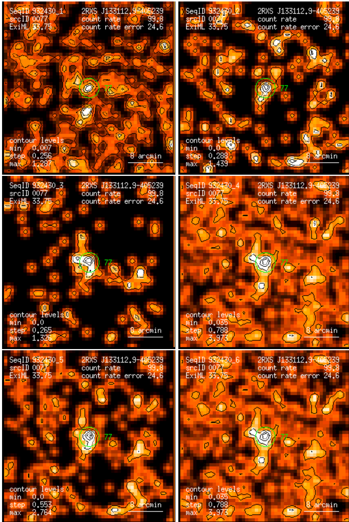
Figure 77: RASS 932430: detection 0077: band rate images, Gaussian filter: (1) PSPC channels 11 – 41, (2) 52 – 90, (3) 91 – 201, (4) 11 – 235, (5) 52 – 201, (6) 11 – 201. Broad band rates in counts/ks. Band rate contour levels in counts/ks/arcmin 2 .
