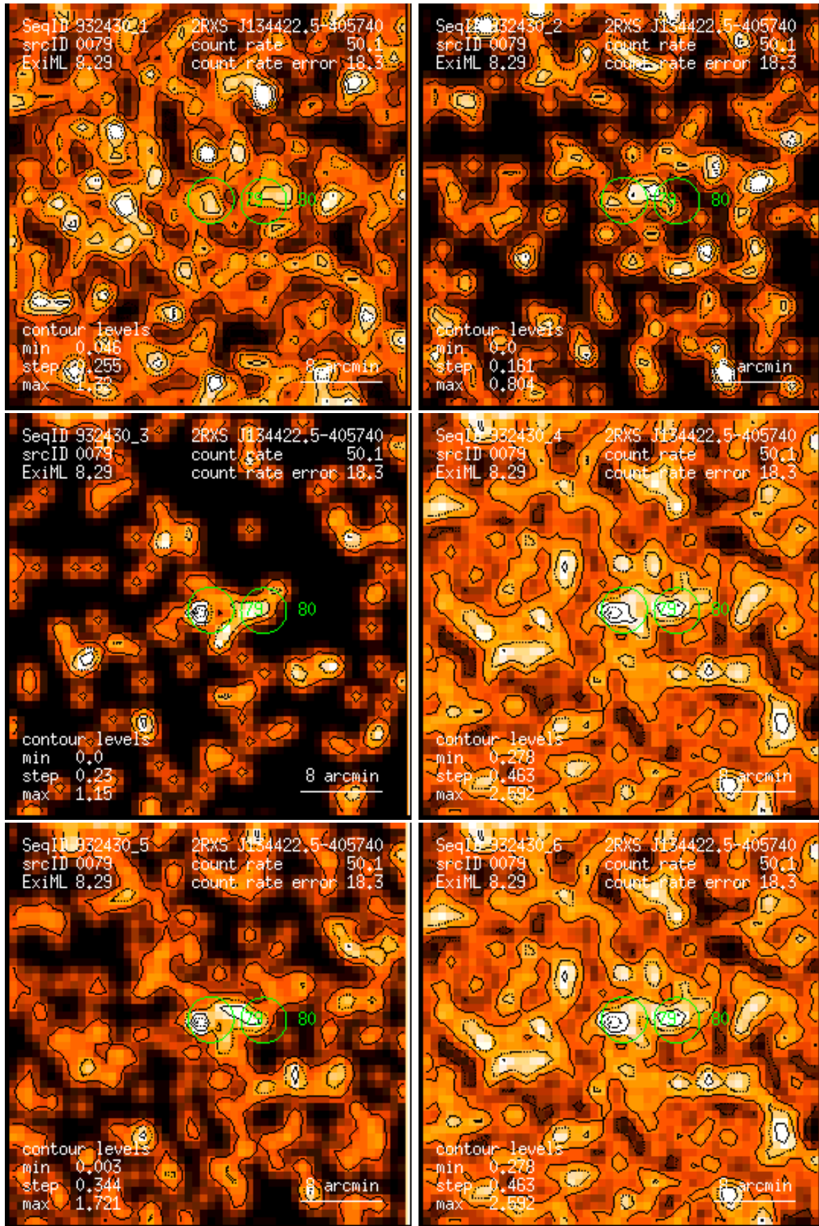
Figure 79: RASS 932430: detection 0079: band rate images, Gaussian filter: (1) PSPC channels 11 – 41, (2) 52 – 90, (3) 91 – 201, (4) 11 – 235, (5) 52 – 201, (6) 11 – 201. Broad band rates in counts/ks. Band rate contour levels in counts/ks/arcmin 2 .
