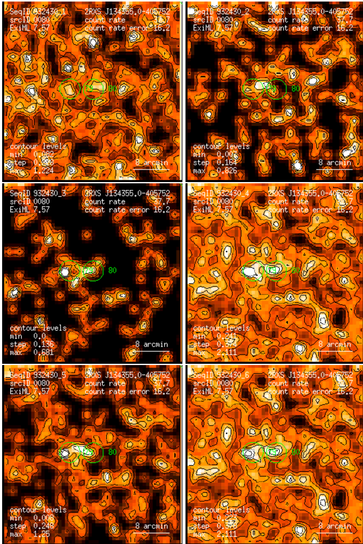
Figure 80: RASS 932430: detection 0080: band rate images, Gaussian filter: (1) PSPC channels 11 – 41, (2) 52 – 90, (3) 91 – 201, (4) 11 – 235, (5) 52 – 201, (6) 11 – 201. Broad band rates in counts/ks. Band rate contour levels in counts/ks/arcmin 2 .
