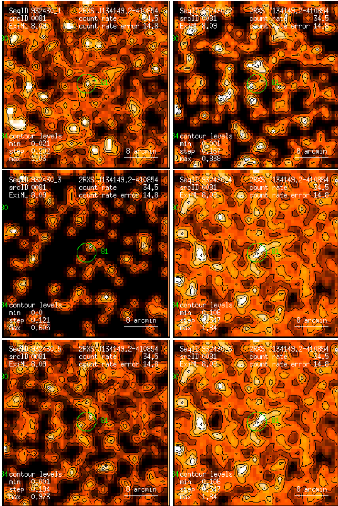
Figure 81: RASS 932430: detection 0081: band rate images, Gaussian filter: (1) PSPC channels 11 – 41, (2) 52 – 90, (3) 91 – 201, (4) 11 – 235, (5) 52 – 201, (6) 11 – 201. Broad band rates in counts/ks. Band rate contour levels in counts/ks/arcmin 2 .
