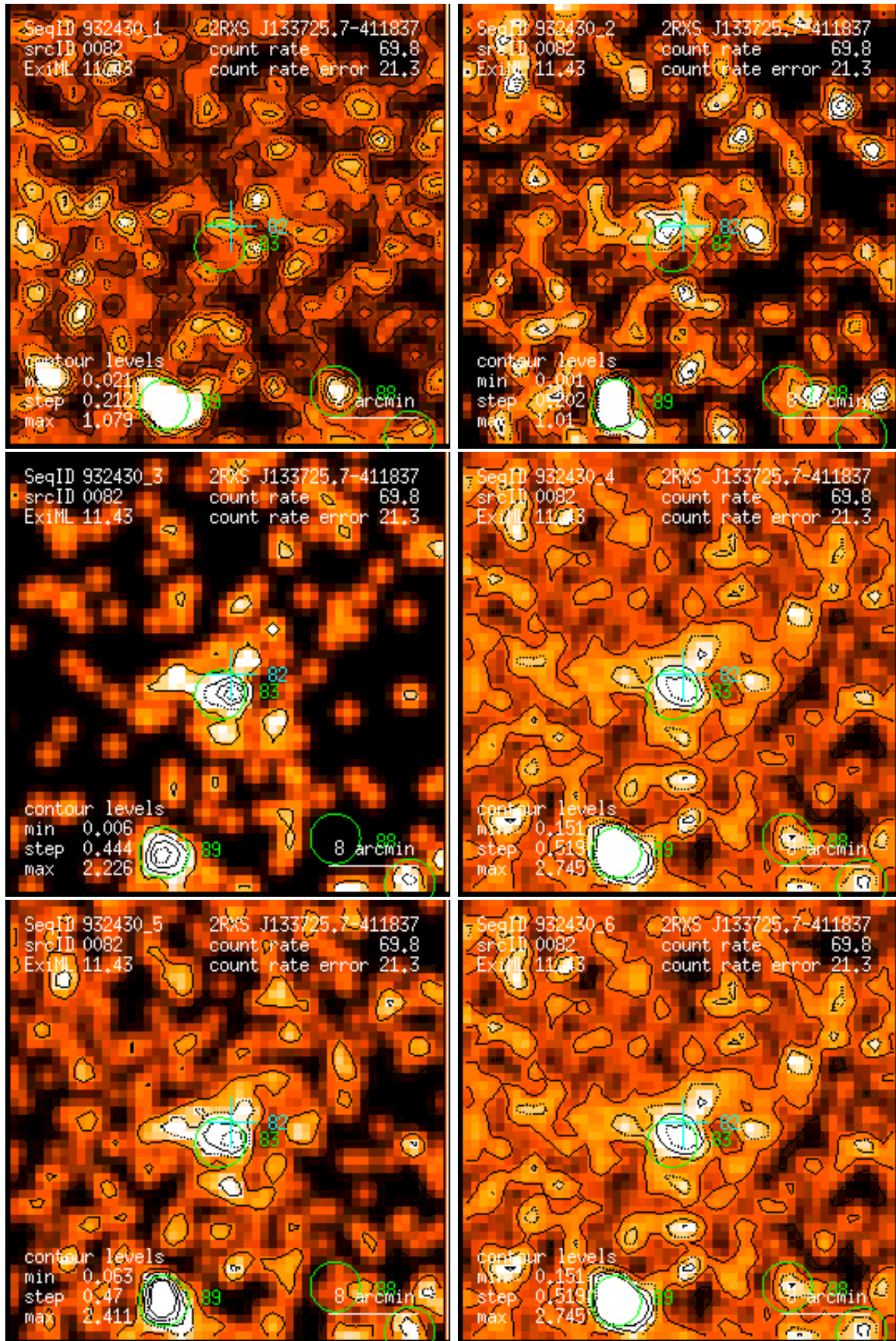
Figure 82: RASS 932430: detection 0082: band rate images, Gaussian filter: (1) PSPC channels 11 – 41, (2) 52 – 90, (3) 91 – 201, (4) 11 – 235, (5) 52 – 201, (6) 11 – 201. Broad band rates in counts/ks. Band rate contour levels in counts/ks/arcmin 2 .
