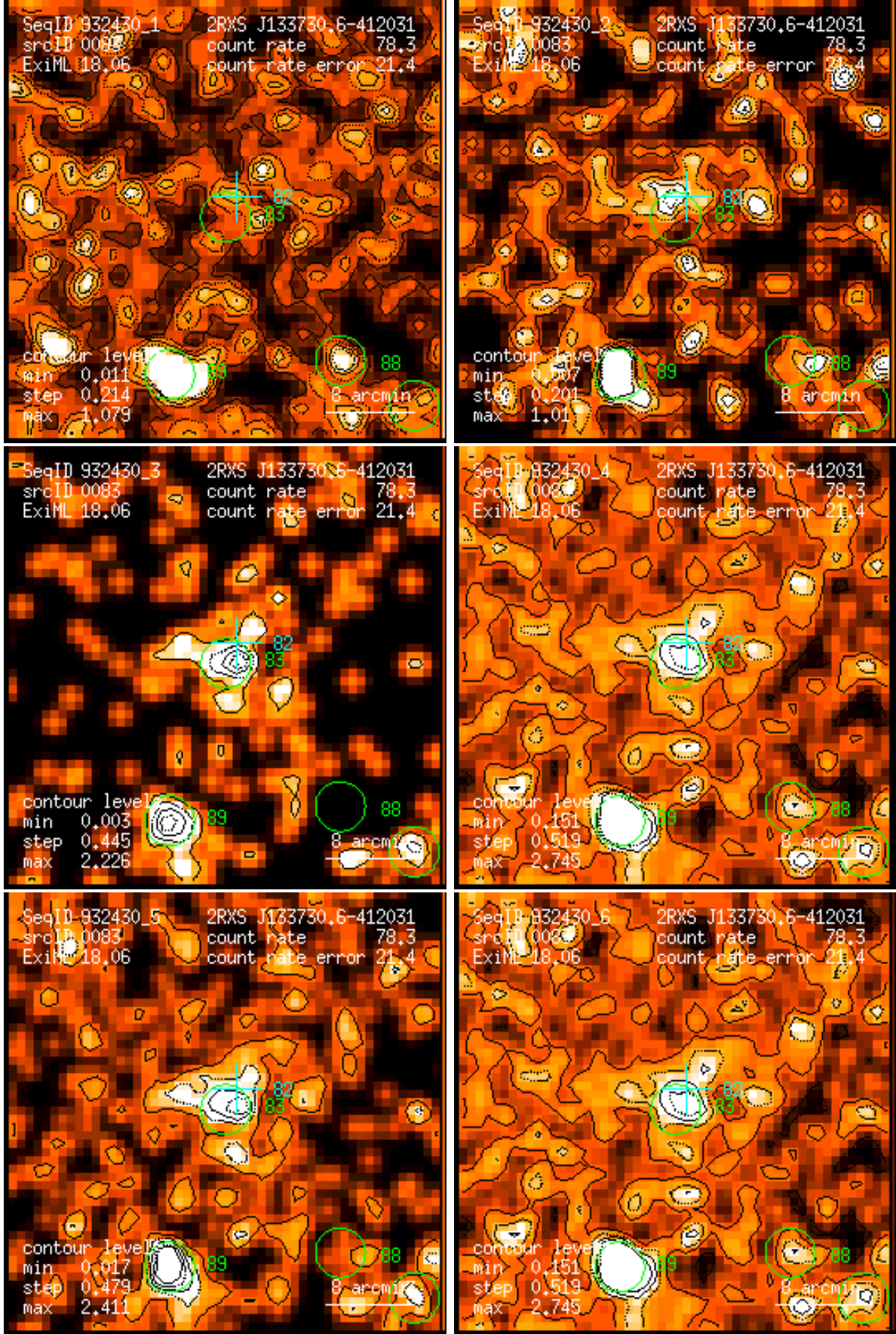
Figure 83: RASS 932430: detection 0083: band rate images, Gaussian filter: (1) PSPC channels 11 – 41, (2) 52 – 90, (3) 91 – 201, (4) 11 – 235, (5) 52 – 201, (6) 11 – 201. Broad band rates in counts/ks. Band rate contour levels in counts/ks/arcmin 2 .
