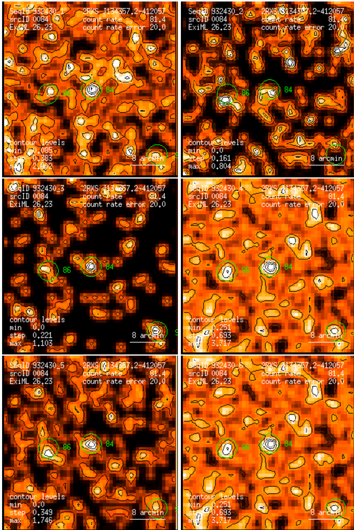
Figure 84: RASS 932430: detection 0084: band rate images, Gaussian filter: (1) PSPC channels 11 – 41, (2) 52 – 90, (3) 91 – 201, (4) 11 – 235, (5) 52 – 201, (6) 11 – 201. Broad band rates in counts/ks. Band rate contour levels in counts/ks/arcmin 2 .
