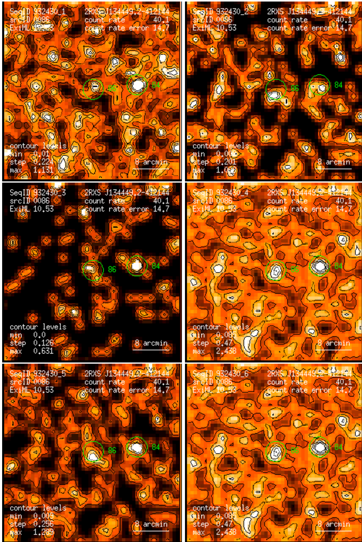
Figure 86: RASS 932430: detection 0086: band rate images, Gaussian filter: (1) PSPC channels 11 – 41, (2) 52 – 90, (3) 91 – 201, (4) 11 – 235, (5) 52 – 201, (6) 11 – 201. Broad band rates in counts/ks. Band rate contour levels in counts/ks/arcmin 2 .
