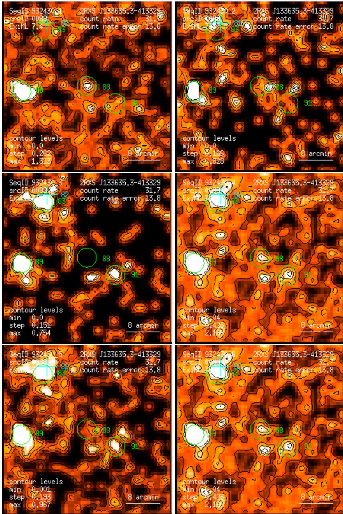
Figure 88: RASS 932430: detection 0088: band rate images, Gaussian filter: (1) PSPC channels 11 – 41, (2) 52 – 90, (3) 91 – 201, (4) 11 – 235, (5) 52 – 201, (6) 11 – 201. Broad band rates in counts/ks. Band rate contour levels in counts/ks/arcmin 2 .
